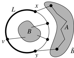
Figure 5: The extension step
