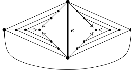
Figure 3: There is no finite peripheral circuit containing the edge e
