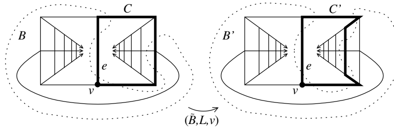
Figure 6: An extension step
