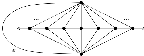
Figure 4: The edge e is not contained in any peripheral circuit
