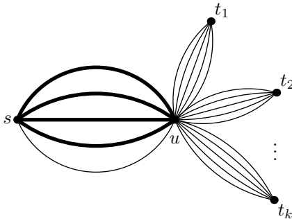
Figure 6: A bad network for nonuniform single source h -flows (for h = 5 ).
