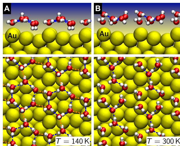
Figure 7. Top and side views of snapshots of an AIMD run of a water layer on Au(511) at (A) T = 140 K and (B) T = 300 K redesigned using the data presented in ref 168. The blue dashed lines indicate the hydrogen bonds, whereas the orange dashed lines in (A) are added in order to emphasize the water structure consisting of tetragons, hexagons, and octagons.
