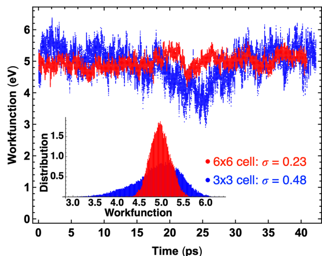
Figure 10. Comparison of the work function of a water film on Pt(111) as a function of the AIMD run time with six water layers in a 3 \times 3 surface unit cell with 36 water molecules 76 and in a 6 \times 6 surface unit cell with 144 water molecules. 23 The inset shows the distribution of the work function values.
