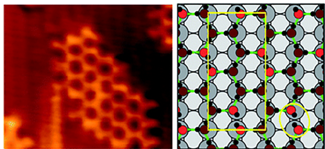
Figure 6. Comparison of an STM image and the calculated structure of the H 2 O–OH c(2 \times 2) phase on Cu(110). Reprinted with permission from ref 163. Copyright 2012 Royal Society of Chemistry. The yellow box indicates the unit cell used in the calculations, and the circle highlights the D-type Bjerrum defect (see text).
