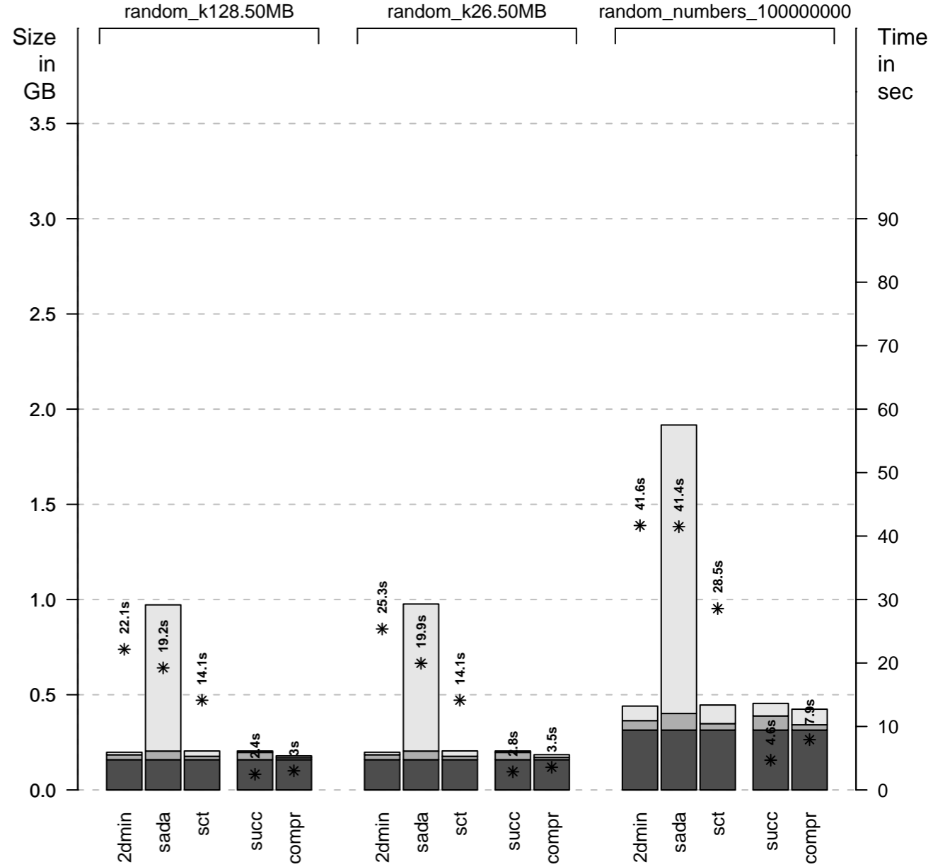
Memory consumption and time for construction
