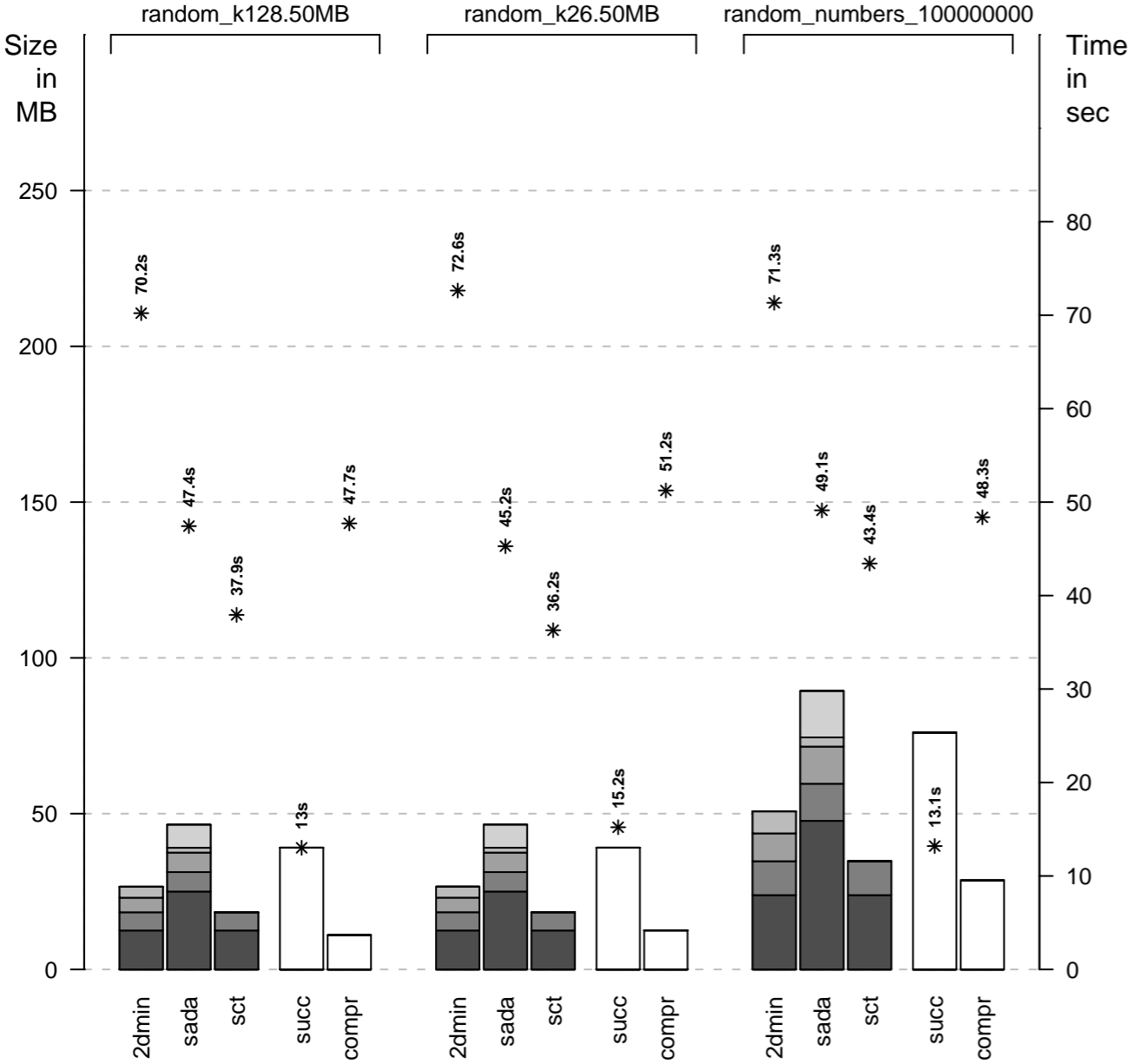
Memory consumption and time for 10^7 queries
