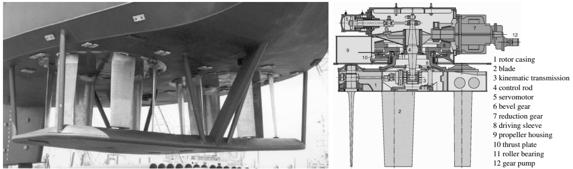
Figure 1: Voith-Schneider® Propeller
