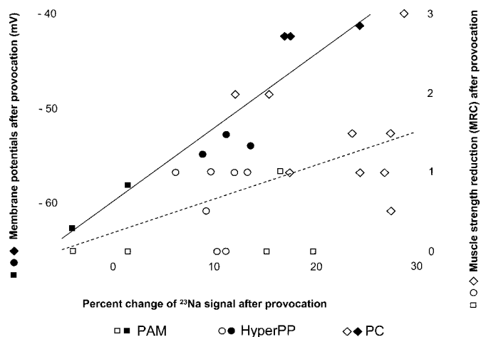
Figure 4. Analysis of the correlation between ^{23}Na signal increase, membrane potential, and muscle strength reduction. The filled symbols represent the mean resting membrane potentials of the muscle fibers taken from the eight patients (three PC, three HyperPP, two PAM) vs the muscular ^{23}Na signal increase of these patients. The open symbols show the decrease in muscle strength of all patients who underwent a provocation test (nine PC, seven HyperPP, five PAM) vs the muscular ^{23}Na signal increase of these patients. The degree of the membrane depolarization correlates with the percent change of the muscular ^{23}Na signal after provocation according to the function y = 0.825x - 60.3 (continuous line) and yields a correlation coefficient of r = 0.92 after Pearson. The muscle strength reduction is much less correlated with the muscular ^{23}Na signal ( r = 0.48 ; y = 0.043x + 0.24 , dashed line for plantarflexion).
