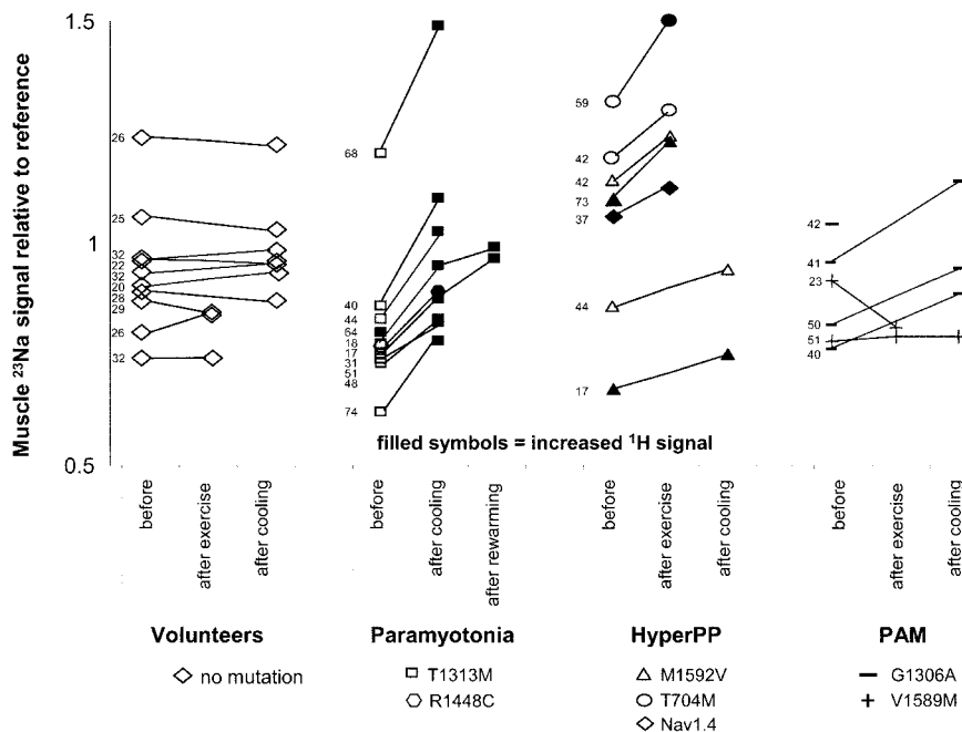
Figure 1. Muscular ^{23}\text{Na} signal intensity relative to reference prior to and after provocation. Muscular ^{23}\text{Na} MRI signal intensities of regions of interest from the lower legs are shown in relation to the signal of the phantom prior to and after provocation. The age of the individual is given in years to the left of the symbols. PC and HyperPP patients exhibited a striking increase in the muscle ^{23}\text{Na} signal intensity after provocation whereas volunteers showed no significant changes. This increase could also be observed in all PAM patients after cooling. A muscle edema was caused by cooling in all PC patients. The 17-year-old HyperPP patient presented with a unilateral calf edema after he had experienced an attack of paresis and aching muscles of this calf 2 days before.
