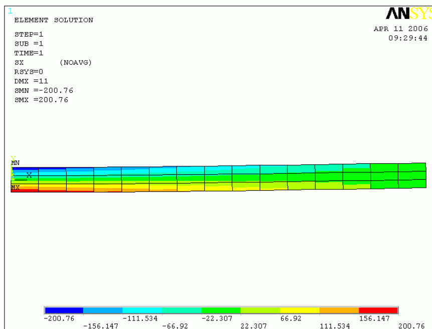
Fig. 25: Contour plot of x-component of stress.
