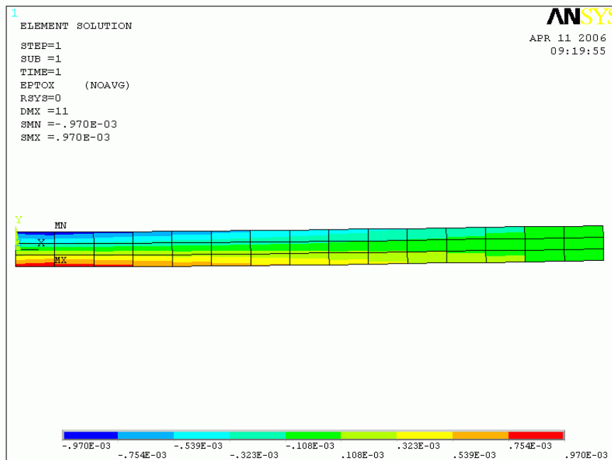
Fig. 24: Contour plot of x-component of total strain.
