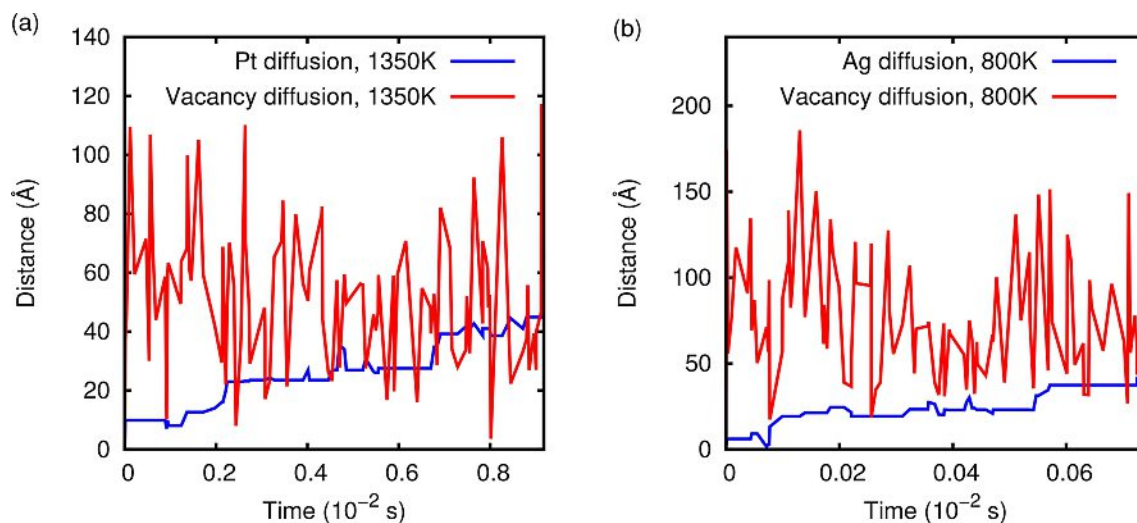
Figure 5. Distance of the foreign atom and the vacancy as a function of time for in total 10^6 kMC steps for the PtRu/Ru(0001) system at 1350 K (a) and for the AgPd(111) system at 800 K (b).
