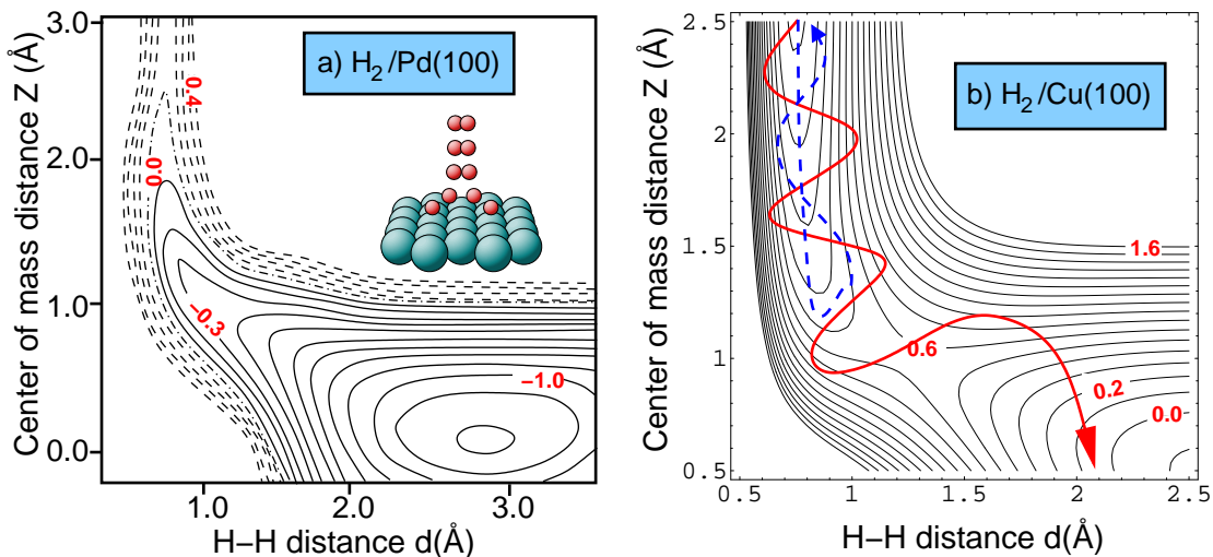
Figure 6: Contour plots of the potential energy surface along two-dimensional cuts through the six-dimensional coordinate space of \text{H}_2 in front of (100) metal surfaces determined by DFT-GGA calculations for \text{H}_2 molecules above the bridge site. The contour spacing is 0.1 eV per \text{H}_2 molecule. (a) \text{H}_2/\text{Pd}(100) (after [43]), (b) \text{H}_2/\text{Cu}(100) [44]. The inset in a) illustrates the process of dissociative adsorption while in b) two typical trajectories showing the effect of initial vibrations are included.
