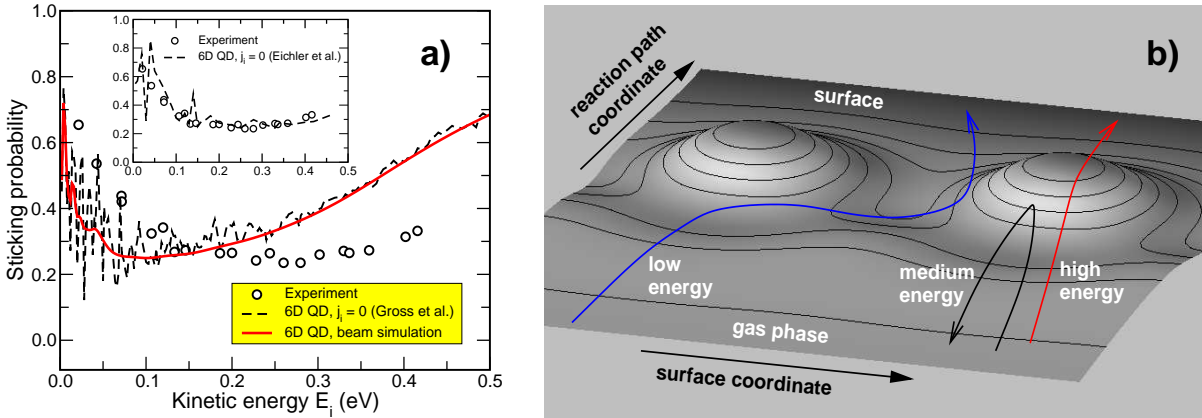
Figure 7: Dissociative adsorption of \text{H}_2/\text{Pd}(100) . a) Sticking probability of \text{H}_2/\text{Pd}(100) as a function of the initial kinetic energy. Circles: experiment [51], dashed and solid line: theory according to \text{H}_2 initially in the ground state and with a thermal distribution appropriate for a molecular beam [49]. The inset shows the theoretical results using an improved ab initio potential energy surface [52]. b) Illustration of the steering effect.
