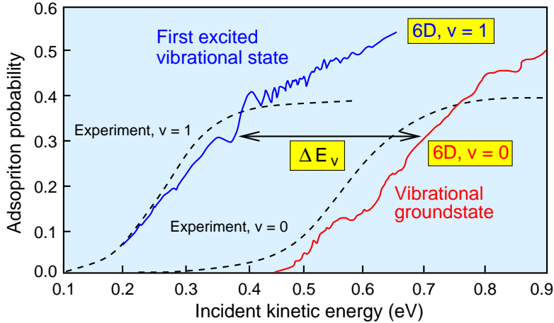
Figure 8: Dissociative adsorption probability of \text{H}_2 on \text{Cu}(100) as a function of the incident kinetic energy determined by six-dimensional quantum wave-packet calculations for molecules initially in the vibrational ground state and first excited state, respectively [61]. The calculations are compared to experimental results derived from an analysis of adsorption and desorption experiments [62].
