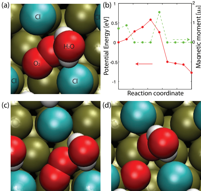
FIG. 5: (a) Atomic structure of the transition state for the dissociation of O 2 superoxo adsorption state on the Pt(111) surface with the presence of H 2 O and Cl - . (b) Potential energy relative to the initial molecular state (solid line) and the magnetic moment (dashed line) during the O 2 dissociation. (c) The initial-state configuration with the O 2 superoxo state. (d) The final-state configuration with atomic O adsorption.
