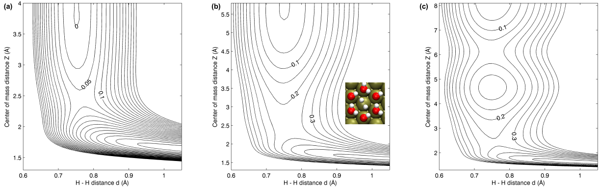
FIG. 6: Two-dimensional cuts through the potential energy surface of the interaction of \text{H}_2 with clean Pt(111) (a) and with Pt(111) covered by one (b) and two (b) water bilayers. The potential energy is plotted as a function of the H–H distance d and the \text{H}_2 center of mass distance Z from the surface. The lateral position and orientation of the \text{H}_2 molecule correspond to a fcc hollow-top-hcp hollow configuration, as indicated in the inset. The contour spacing in (a) is 25 meV, while it is 50 meV in (b) and (c). Note the different scales of the Z axis.
