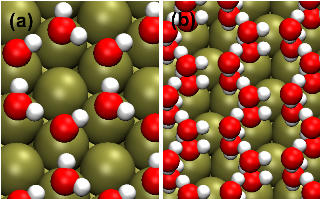
FIG. 1: Illustration of the most stable water structures on Pt(111) according to the DFT calculations. a) H-down bilayer structure, b) H-down double bilayer structure.
