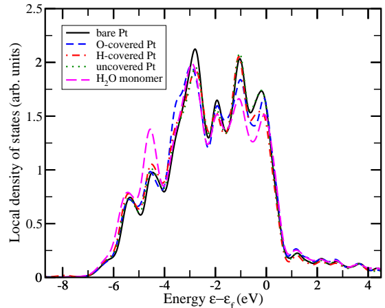
FIG. 2: Local density of states (LDOS) of the Pt(111) surface atoms without and in the presence of water. For the adsorption of a single water molecule, only the LDOS of the Pt atom directly below the water molecule is plotted, whereas for the H-down water bilayer the LDOS of the three inequivalent Pt atoms within the surface unit cell is shown.
