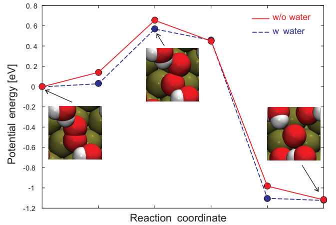
FIG. 4: Potential energy along the O_2 dissociation path on Pt(111) with and without water starting from the nonmagnetic molecular precursor state of O_2 .
