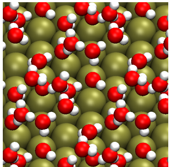
FIG. 7: Illustration of a disordered water structure considered in the calculations with two water molecules extracted from the lower water layer and three from the upper.
