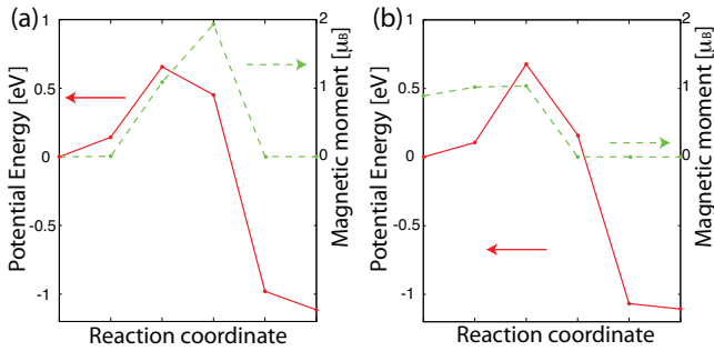
FIG. 3: The total energy relative to the initial molecular state (solid line) and the magnetic moment (dashed line) during the O_2 dissociation for (a) peroxo and (b) superoxo adsorption states on the Pt(111) surface.
