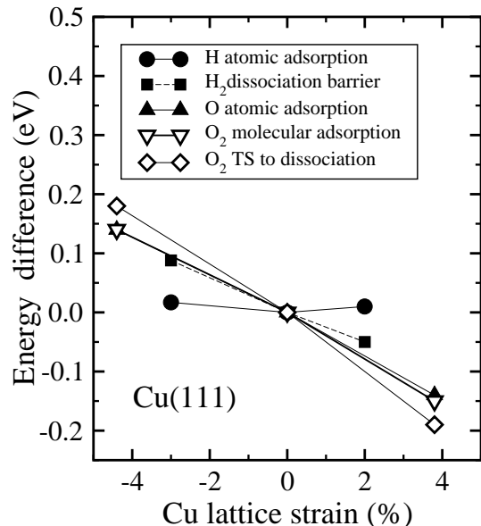
FIG. 8: Change of the hydrogen adsorption energy and dissociation barrier and the oxygen atomic and molecular adsorption energies as well as the transition state (TS) to dissociation on Cu(111) as a function of the lattice constant. The data for oxygen are taken from Ref. [6].
