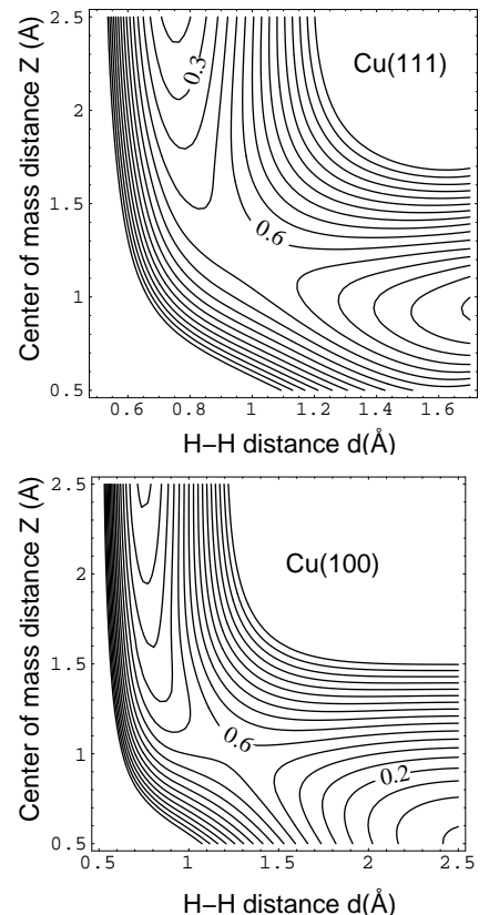
FIG. 6: Potential energy surface for the hydrogen dissociation on Cu(111) and Cu(100) as a function of the H-H interatomic distance d and the center of mass distance from the surface Z . The energy is in eV/molecule, the energy spacing of the contour lines is 0.1 eV. The dissociation path corresponds to the h-b-h geometry, i.e., the center of mass has been kept fixed laterally above the bridge site with the hydrogen atoms dissociating into the neighboring three- or fourfold hollow sites, respectively. Note the different scale of the d axes.
