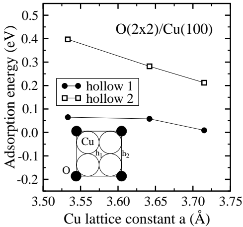
FIG. 5: Atomic hydrogen adsorption energies as a function of the lattice strain at the hollow sites of the O(2\times 2)/Cu(100) surface. The adsorption sites are indicated by h_1 and h_2 in the inset.
