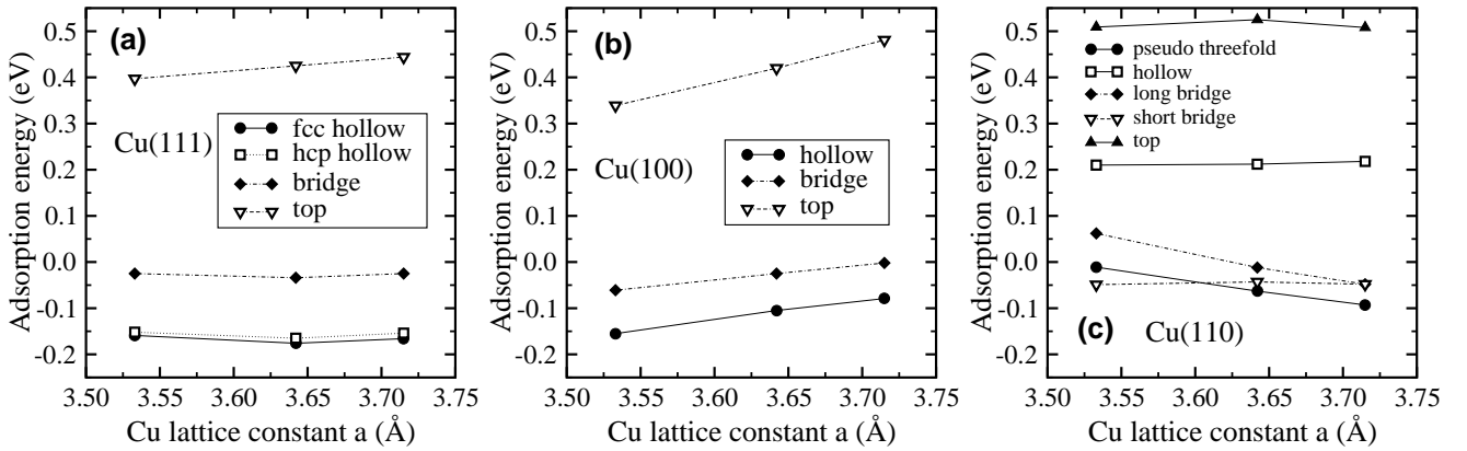
FIG. 3: Atomic hydrogen adsorption energies as a function of the lattice strain at the high-symmetry points of (a) Cu(111), (b) Cu(100), (c) Cu(110).
