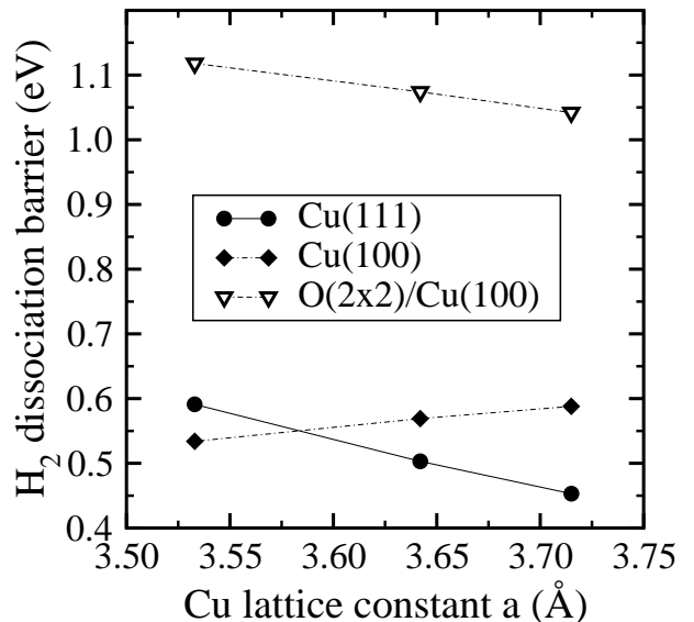
FIG. 7: The H_2 dissociation barrier in the h-b-h geometry (see text) on Cu(111), Cu(100) and O(2×2)/Cu(100) as a function of the lattice strain.
