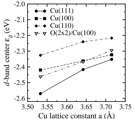
FIG. 2: The d -band center \varepsilon_d of the surface layer with respect to the Fermi energy as a function of the lattice strain for different copper surface terminations
