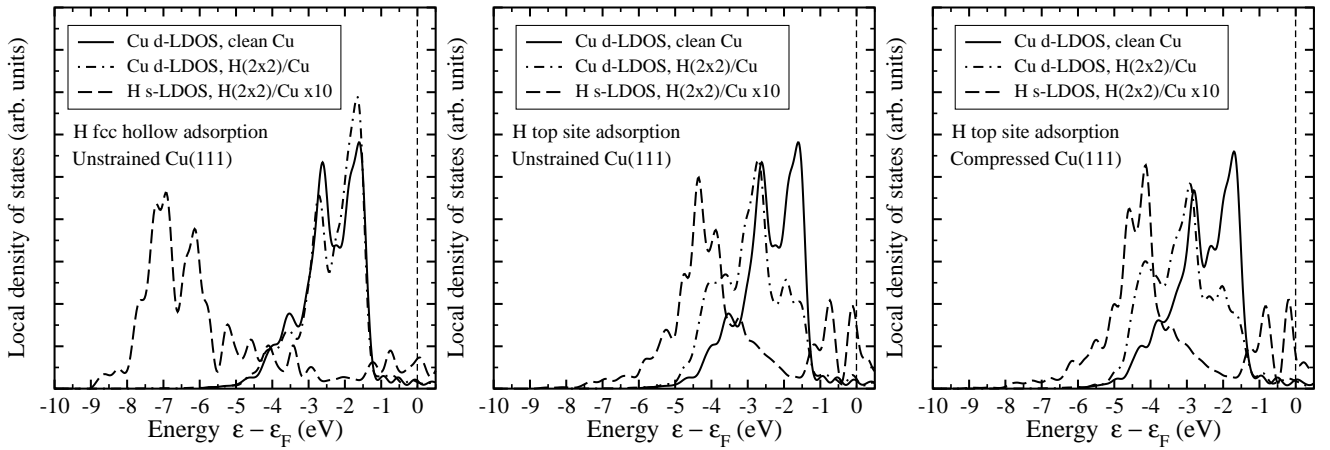
FIG. 4: Local density of states of the hydrogen 1s state and the Cu d -band for atomic hydrogen adsorption on unstrained Cu(111) at the fcc hollow site (a) and the top site (b) and at the top site for compressed Cu(111) (c). The hydrogen 1s density of states is multiplied by a factor of ten.
