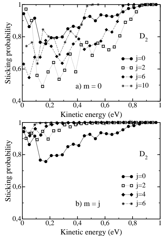
FIG. 3: Three-dimensional calculation of the sticking probability of D_2 for a range of initial rotational states j as a function of the kinetic energy. a) Molecules initially rotating in the cartwheel fashion m = 0 , b) molecules initially rotating in the helicopter fashion m = j .
