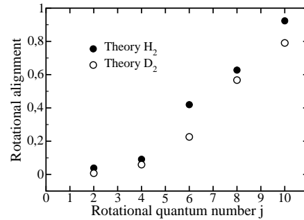
FIG. 6: Three-dimensional quantum results of the rotational alignment of hydrogen molecules desorbing from Pd(100) at a surface temperature T_s = 700\text{K} with the hydrogen bond length and moment of inertia kept frozen at their gas phase values.
