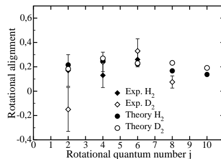
FIG. 8: Comparison of the rotational alignment of H_2 and D_2 molecules desorbing from Pd(100) at a surface temperature T = 700K derived from five-dimensional quantum calculations (circles) with the experimental results [8, 31] (diamonds). Filled symbols: H_2 , open symbols: D_2 .
