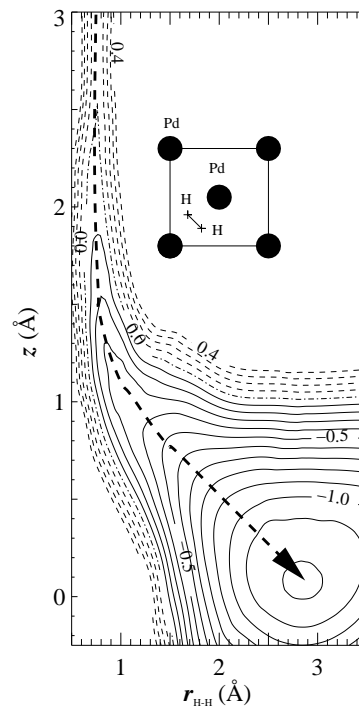
FIG. 1: Two-dimensional cut through the six-dimensional potential energy surface of \text{H}_2/\text{Pd}(100) obtained by density functional calculations [21]. The coordinates in the figure are the \text{H}_2 center-of-mass distance from the surface z and the H-H interatomic distance r . Energies are in eV per \text{H}_2 molecule. The contour spacing is 0.1 eV. The lateral coordination and the orientation of the molecule are illustrated in the inset. The dashed line corresponds to the reaction path.
