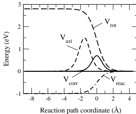
FIG. 2: The functions V_{\text{reac}}(s) , V_{\text{rot}}(s) , V_{\text{azi}}(s) and V_{\text{corr}}(s) describing the most favorable reaction path, the anisotropy and the corrugation of the model potential energy surface used in the calculations.
