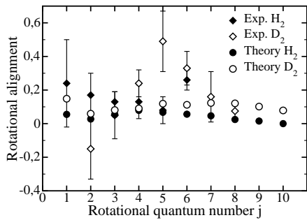
FIG. 5: Rotational alignment of H 2 and D 2 molecules desorbing from Pd(100) at a surface temperature T = 700\text{K} . Diamonds correspond to the experimental results [8, 31] while three-dimensional quantum results are plotted as circles. Filled symbols: H 2 , open symbols: D 2 .
