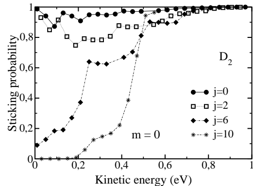
FIG. 4: Three-dimensional calculation of the sticking probability of \text{D}_2 for a range of initial rotational states j as a function of the kinetic energy for molecules initially rotating in the cartwheel fashion m = 0 . The D-D bond length and consequently the \text{D}_2 moment of inertia are kept frozen at their gas phase values.
