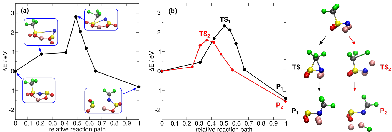
FIG. 6. Minimum energy paths of intramolecular rearrangements of (a) \text{LiN}(\text{SO}_2)(\text{SO}_2\text{CF}_3) or (b) \text{Li}_2\text{NSO}_2\text{CF}_3 in which the S-C bond is broken and a N-C bond is formed.
