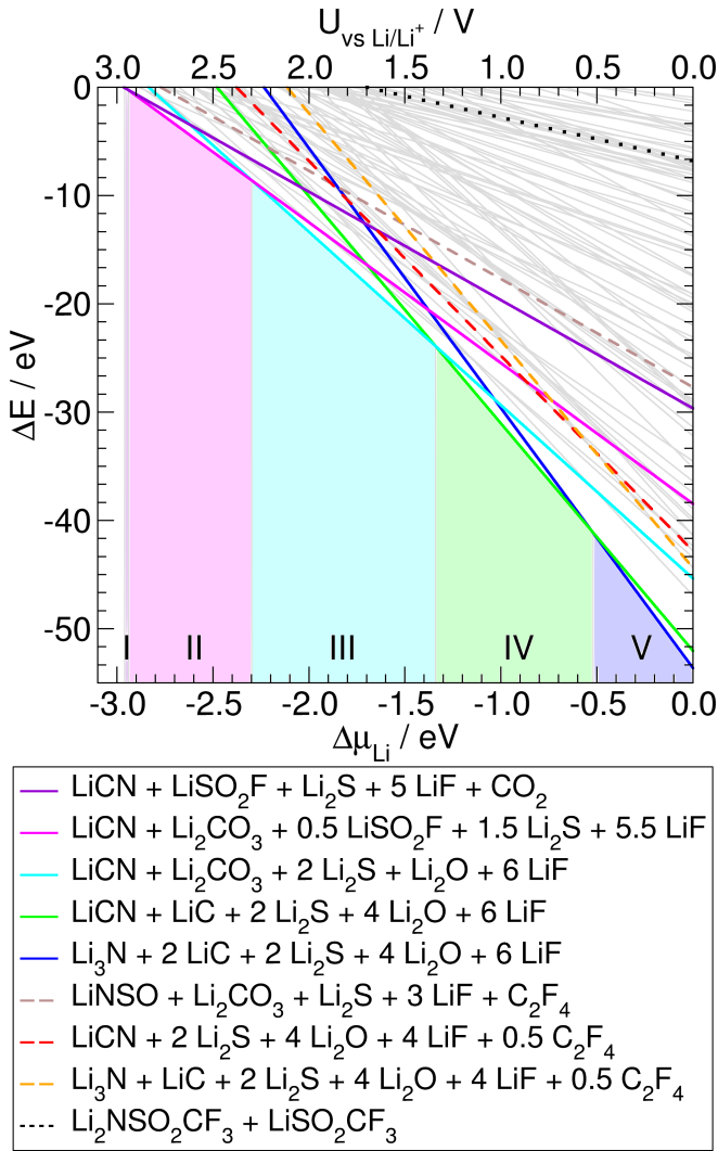
FIG. 4. Reaction energies \Delta E as a function of the chemical potential of Li ( \Delta\mu_{\text{Li}} ) or of the electrode potential ( U vs \text{Li}/\text{Li}^+ ) according to ???. Colored solid lines mark the most stable products. Colored dashed lines highlight the most stable products of reactions including evolution of \text{C}_2\text{F}_6 or \text{C}_2\text{F}_4 . The respective products are denoted in the legend. The black dotted line denotes the reaction to \text{Li}_2\text{NSO}_2\text{CF}_3 and \text{LiSO}_2\text{CF}_3 as possible model for the initial reaction. The grey lines correspond to other possible product combinations that were considered.
