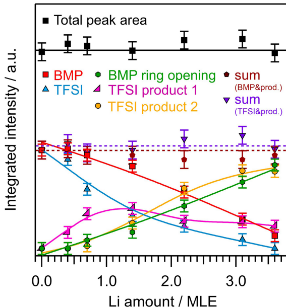
FIG. 3. Quantitative analysis of the integrated peak intensities in the N 1s core level region vs. Li coverage.
