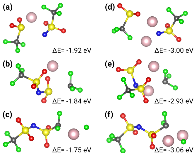
FIG. 5. Products and energies of the reaction of \text{TFSI}^- and one Li atom (a-c) or two Li atoms (d-f) involving N-S bond breaking (a, d), S-C bond breaking (b, e) or C-F bond breaking (c, f). The reaction energies \Delta E are given per Li atom and referred to the energies of an isolated \text{TFSI}^- anion and an isolated Li atom calculated by employing the implicit solvation model CPCM.
