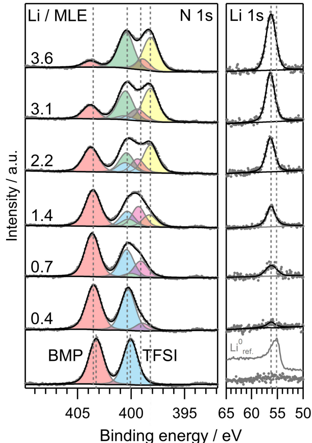
FIG. 1. N 1s and Li 1s core level spectra of around 10 ML of molecularly adsorbed BMP-TFSI species (bottom of the N 1s region) and after stepwise post-deposition of 0.4 - 3.6 MLE of Li at r.t. For comparison, a reference spectrum for metallic Li is included in the Li 1s range.
