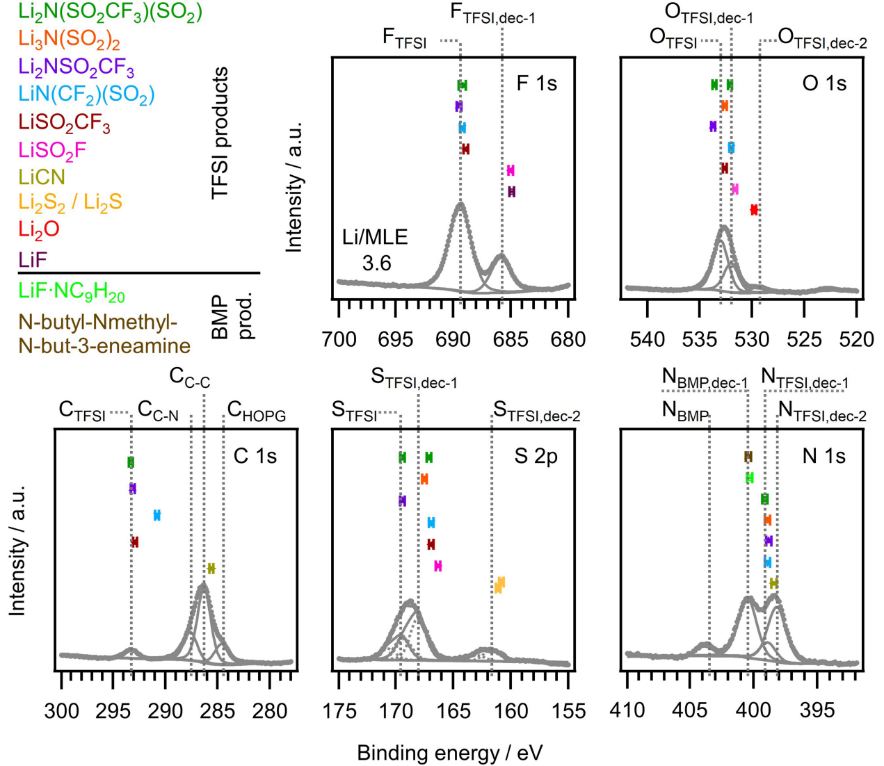
FIG. 7. F 1s, O 1s, C 1s, S 2p and N 1s core level spectra of an adsorbed BMP-TFSI multilayer ( \sim 10 ML) after post-deposition 3.6 ML Li (bottom of each panel). The calculated BEs of several fragments are inserted as markers in the panels (error bar \pm 0.2 eV).
