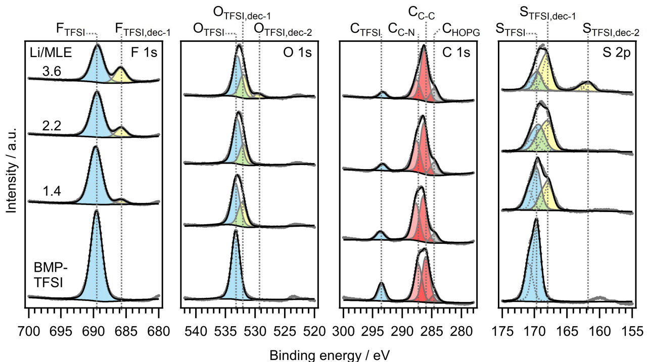
FIG. 2. F 1s, O 1s, C 1s and S 2p core level spectra of an adsorbed BMP-TFSI multilayer ( \sim 10 ML) and after stepwise post-deposition of 1.4, 2.2 and 3.6 MLE of Li at r.t.
