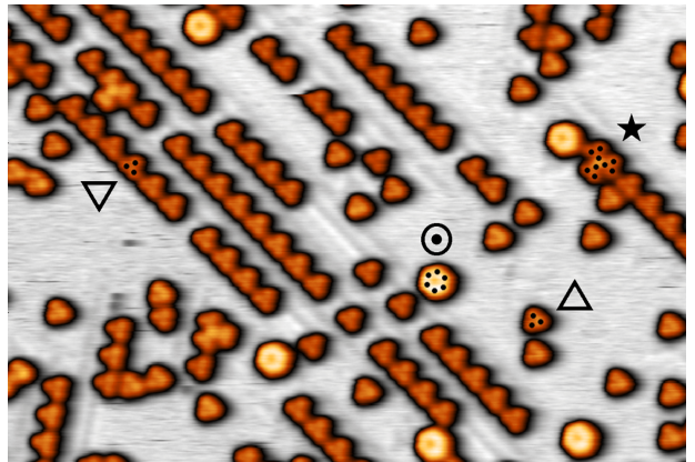
FIG. 2: (Color online) Atomically resolved STM image (image size 200 Å \times 135 Å) of Ni micro-islands created by oxygen adsorption (exposure about 6 L at T_{oxygen} = 400 K) on a densified, moiré-distorted Ni monolayer on Ru(0001) ( \Theta_{Ni} = 0.9 ML, T_{growth} = 350 K) [9]. Four types of micro-islands can be distinguished: upside-down trimers arranged along rows ( \nabla ); isolated trimers oriented upright ( \triangle ); donut-shaped hexagons consisting of 6 Ni-atoms ( \odot ); star-like arrangements of three trimers ( \star ).
