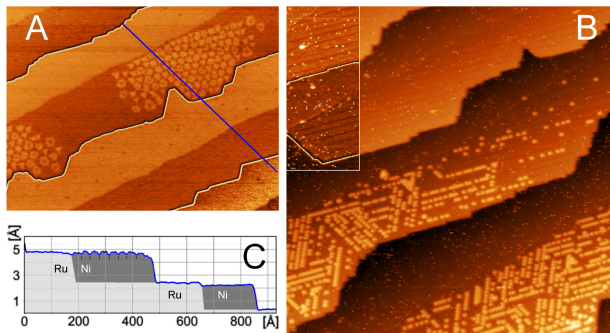
FIG. 1: (Color online) STM images of Ni deposited onto Ru(0001) ( \Theta_{Ni} = 0.6 ML, T_{growth} = 373 K) before (A) and after (B) oxygen has been adsorbed (exposure about 15 L at T_{oxygen} = 400 K) [9]. A line scan across Ru step edges and deposited Ni, as indicated by the line in (A), is displayed in (C). In (A), extended areas of the Ni monolayer lead to a loss of the pseudomorphic structure and the formation of a moiré overstructure of the Ni film (periodicity \delta a \approx 30\text{-}35 Å as indicated by the markers in (C), corrugation \delta z \approx 0.3 Å). The color scheme of image (B) has, in part, been adjusted (inset) to clearly display the uniaxial distortion of the Ni monolayer if oxygen is adsorbed. STM image sizes: (A) 1200 Å \times 900 Å; (B) 830 Å \times 830 Å.
