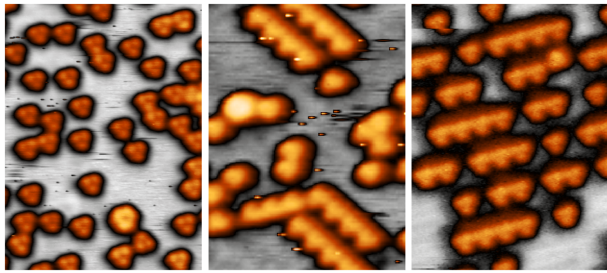
FIG. 4: (Color online) STM images ( 70 \text{ \AA} \times 100 \text{ \AA} each) of Ni deposited onto Ru(0001) ( \Theta_{Ni} = 0.9 \text{ ML} , T_{growth} = 400 \text{ K} ) which has been exposed to increasing amounts of oxygen at T_{oxygen} = 400 \text{ K} [9]: (left) Oxygen exposure 1 L; (center) additional oxygen exposure 2 L; (right) additional oxygen exposure 10 L. In between of the gas exposures the sample has been recooled to room temperature for STM imaging.
