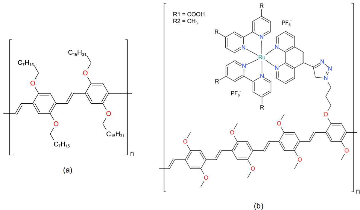
Figure 2: (a) Structure of PPV polymer; alkyl chains are replaced by methyl groups to reduce the computational cost. (b) Unit cells used in the periodic DFT calculations to model the polymer and the Ru(II) dye linked to the polymer. Structure of the Ru(II)-based photosensitizer linked to the PPV polymer (PPV-Ru) together with two \text{PF}_6^- counter ions for charge balancing. Two different substituents have been used, \text{R}=\text{COOH} and \text{R}=\text{CH}_3 , yielding the hybrid materials PPV-Ru1 and PPV-Ru2, respectively.
