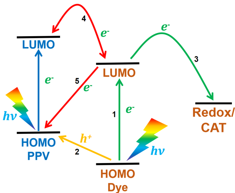
Figure 1: Schematic presentation of the processes occurring in p-DSSC solar cell of a photoactive complex coupled to a PPV polymer.
