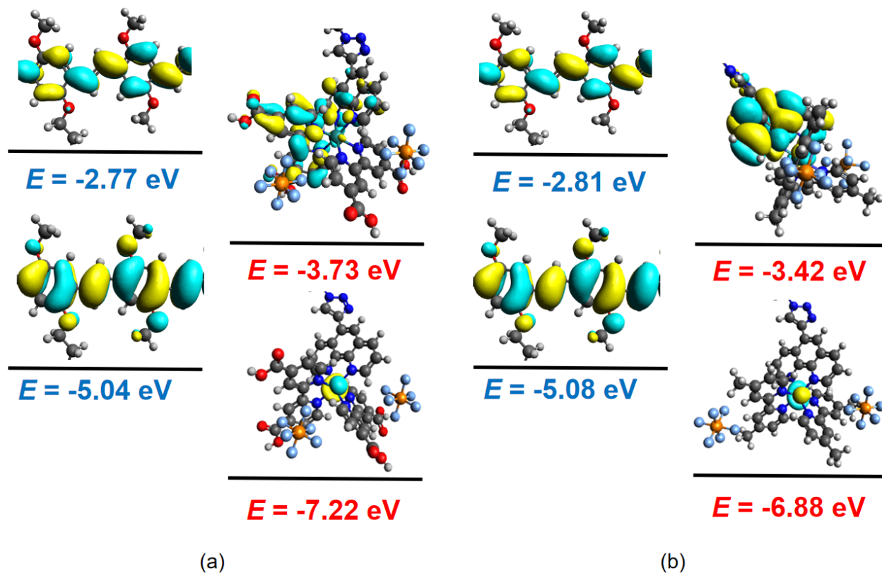
Figure 4: HOMO and the LUMO levels of the PPV polymer and the Ru photosensitizer with the -\text{COOH} (a) and -\text{CH}_3 (b) substituents, respectively, in the gas phase taken with respect to the electronic vacuum level. The numbers in blue represent the HOMO-LUMO levels of PPV, those in red color denote the HOMO-LUMO levels of the photosensitizer. These levels have been identified through a charge analysis of the electronic orbitals which is illustrated by the charge isosurfaces in the ball-and-stick presentation of the polymer and the Ru photosensitizer.
