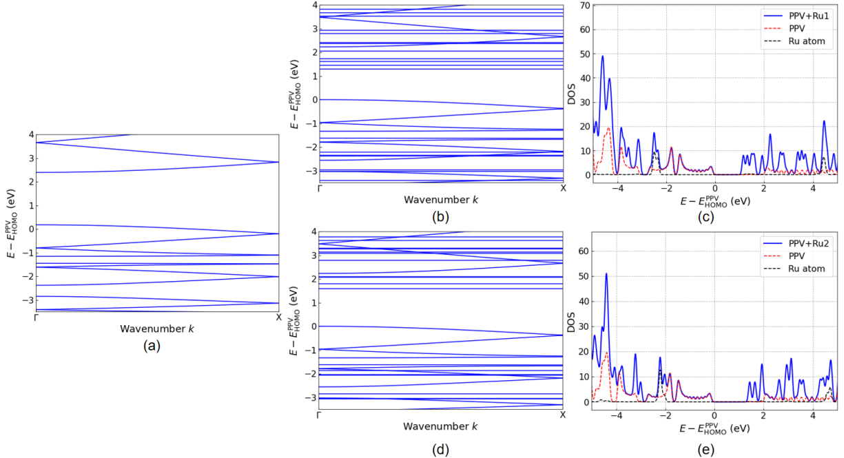
Figure 3: Bandstructures and densities of states of the PPV polymer alone and coupled to the Ru photosensitizer with -\text{COOH} (PPV-Ru1) and -\text{CH}_3 (PPV-Ru2) substituents in the gas phase calculated with the PBE0 functional. a, b, d) Band structure of the isolated PPV polymer, the PPV-Ru1 and the PPV-Ru2 systems, respectively; c, e) density of the states (DOS) of the PPV-Ru1 and the PPV-Ru2 systems, respectively. In the presentation of the DOS, a smearing of 50 meV has been applied.
