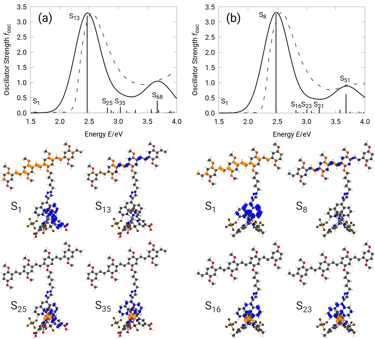
Figure 8: Visualization of calculated UV/absorption spectra (solid) and excitations for PPV-Ru1 (a) and PPV-Ru2 (b). Experimental spectra (dashed) are adapted from ref. 15 and have been scaled arbitrarily. Calculated transitions have been broadened to a full width at half maximum of 0.5 eV. Charge density difference plots (isovalue = 0.002) for some important transitions are included. Holes are depicted in orange, electrons in blue. Calculated data was obtained at the PBE0/def2-SVP level of TDDFT. Energies and oscillator strengths can be found in Tab. 3.
