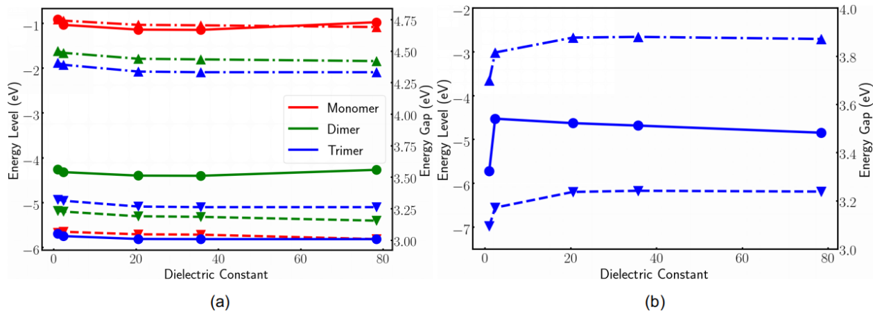
Figure 5: Energy levels of the HOMO (▲), the LUMO (▼), and the energy gap (●) of isolated PPV oligomers and the Ru2 dye as a function of the dielectric constant of an implicit solvent they are embedded in.
