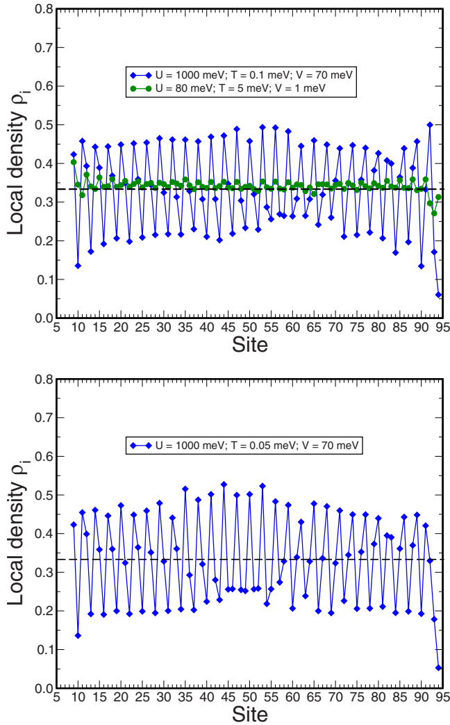
FIG. 11. (Color online) Local densities \rho_i of a chain with length L=102 and a coverage of \rho=\frac{1}{3} obtained from DMRG calculations for two different sets of parameters given in the legend.
