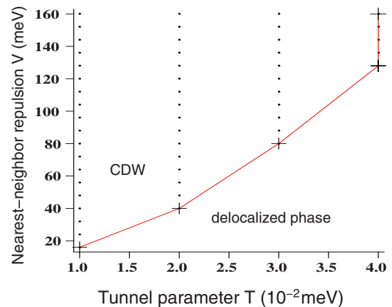
FIG. 4. (Color online) Phase diagram for half filled chains as a function of the tunnel parameter T and the nearest-neighbor repulsion V with an on-site repulsion of U=1000 meV. The small dots denote systems in which a CDW phase has been found.
