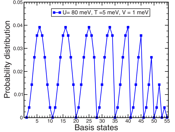
FIG. 1. (Color online) Probability distribution of finding one of the 55 basis states in the expansion of the ground state. See the text for an explanation of the ordering of the basis states.
