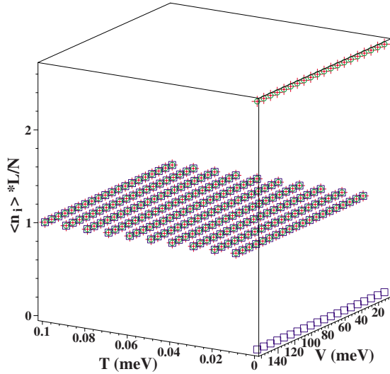
FIG. 5. (Color online) Renormalized local densities \rho_1 \equiv crosses, \rho_2 \equiv squares, and \rho_3 \equiv circles over T and V for L=8 , N=3 , and U=1000 meV.
