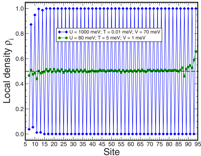
FIG. 9. (Color online) Local densities \rho_i of a chain with length L=100 and a coverage of \rho=\frac{1}{2} obtained from DMRG calculations for two different sets of parameters given in the legend. 15 states and three sweeps were used.
