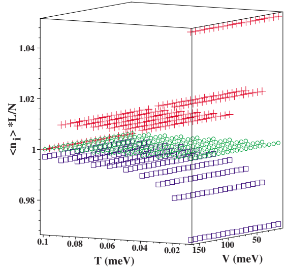
FIG. 6. (Color online) Renormalized local densities \rho_1 \equiv crosses, \rho_2 \equiv squares, and \rho_3 \equiv circles as a function of the tunnel parameter T and the nearest-neighbor repulsion V for L=8 and N=3 with a perturbation \varepsilon=0.0005 meV at site 1.
