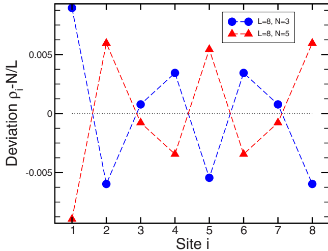
FIG. 8. (Color online) Deviation \delta_i of a chain of length L=8 with particle densities \rho=3/8 and 5/8 and perturbations according to Eq. (12) with \varepsilon=0.0005 meV and \varepsilon=-0.0005 meV, respectively. The remaining parameters are U=1000 meV, T=0.02 meV, and V=70 meV.
