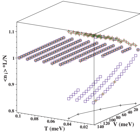
FIG. 2. (Color online) Renormalized local densities \rho_1 \equiv crosses, \rho_2 \equiv squares, and \rho_3 \equiv circles over T and V for L=8 , N=4 , and U=1000 meV. The black line is the projection line of the phase boundary into the V - T plane.
