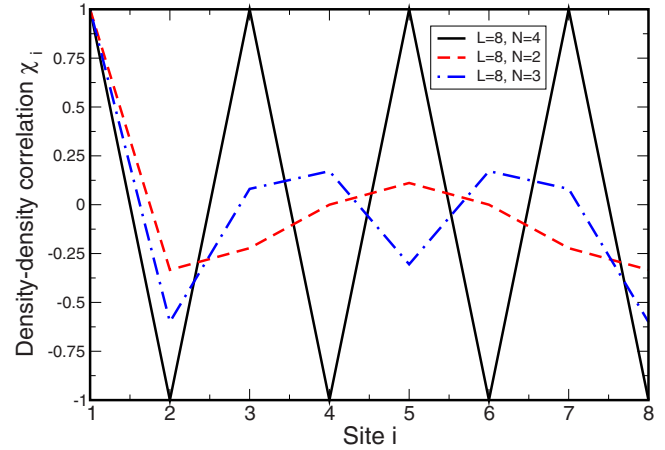
FIG. 3. (Color online) Normalized density-density correlation function \chi_i [Eq. (11)] for L=8 and N=2, 3, 4 . The particular parameters are U=1000 meV, T=0.02 meV, and V=70 meV.
