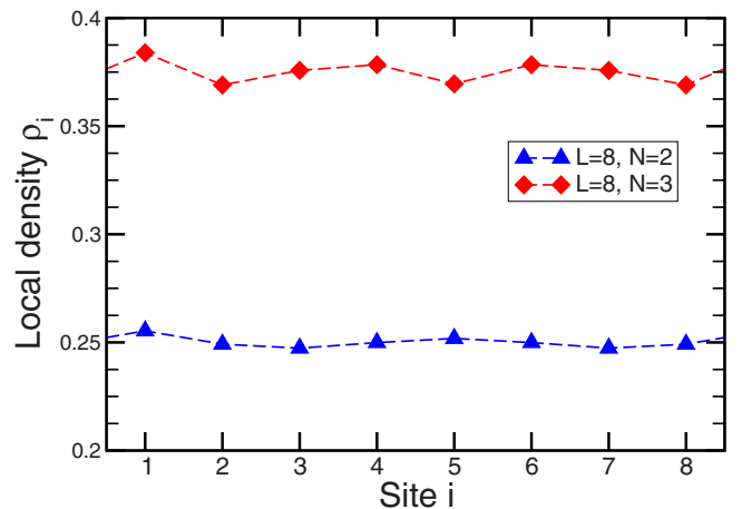
FIG. 7. (Color online) Local densities \rho_i, i=1, \dots, 8 , of a chain of length L=8 occupied by N=2 and N=3 particles ( T=0.02 meV, V=70 meV, and U=1000 meV) with a perturbation \varepsilon=0.0005 meV at site 1.
