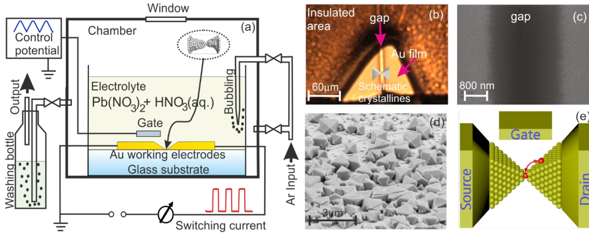
FIG. 1. Scheme of the experimental setup to fabricate Pb atomic-scale transistors, surface analysis and the model of a single-atom transistor. (a) Pb is deposited and dissolved electrochemically in the narrow gap between two gold working electrodes on a glass substrate, and the conductance of the contact is measured simultaneously. The potentials of the working electrodes with respect to the lead reference electrode and the lead counter electrode are set by a potentiostat. (b) Confocal optical microscope image of as-prepared Au electrodes. The Au electrodes were insulated with a polymer film except for a shining triangle range for the electrochemical deposition of Pb. A schematic diagram of two Pb microcrystallines in grey is placed across the gap between the two gold electrodes to illustrate a point-contact formation. (c) Scanning electron microscopy image of a shadow-sputtered gap. (d) Scanning electron microscopy image of deposited Pb microcrystals on the Au electrodes. (e) Schematic model of a single-atom transistor.
