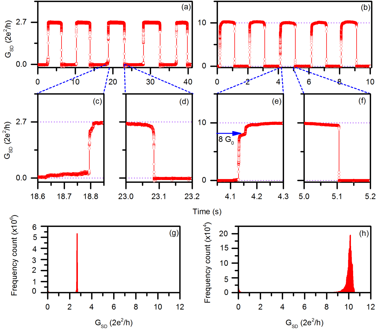
FIG. 5. Detailed comparison of two switching sequences, (a) 0– 2.7 G_0 and (b) 0– 10 G_0 . The data of the two sequences was recorded at a sampling rate of 50,000 1/s. Graphs (a) and (b) show only 5 cycles for each switching, the small empty circles indicate measured data, and the lines are guidance for the eye. Graphs (c), (d), (e), and (f) display closing and opening events of the 3 rd cycle in each sequence, respectively. The conductance histogram for each switching sequence of 68 cycles in total is presented in (g) and (h), respectively. The full width at half maximum is 0.06 G_0 around 2.67 G_0 , and 0.30 G_0 around 10.13 G_0 . For the histograms, the fast-recorded conductance data was collected in bin sizes of 0.02 G_0 .
