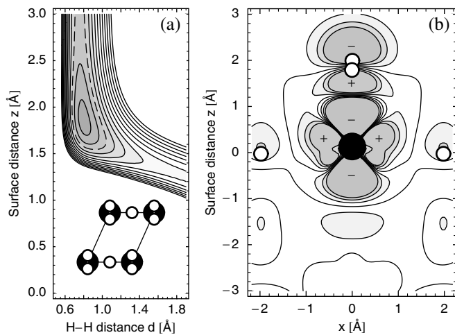
FIG. 4. DFT results of the \text{H}_2 molecular adsorption on the hydrogen-covered Pd(210) surface. (a) Contour plot of potential energy surface. The coordinates in the figure are the \text{H}_2 center-of-mass distance from the surface z and the H-H interatomic distance d . The lateral H coordinates are indicated in the inset. The contour spacing is 0.1 eV, and the vacuum energy level is marked by the dashed contour line. (b) Electron density difference plot of the molecular adsorption state in the x - z plane. The positions of the H atoms and the top Pd atom are marked by open and filled circles, respectively.
