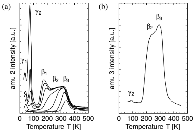
FIG. 2. Thermal desorption spectra. (a) Series of H_2 TPD spectra for different exposures between 0.02 and 0.2 L at a temperature of 50 K. (b) Mass 3 (HD) TPD spectrum after a mixed H_2/D_2 exposure at 50 K.
