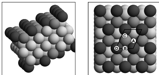
FIG. 1. Side and top view of the (210) surface. In the right panel the surface unit cell plus the three atomic adsorption sites A, B, and C are included. The site D corresponds to the molecular adsorption site.
