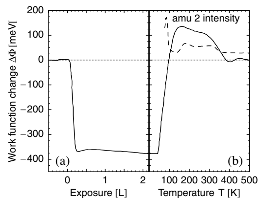
FIG. 3. Hydrogen-induced work function change \Delta\Phi . (a) Dependence of \Delta\Phi on H_2 exposure for adsorption at 50 K. (b) Dependence of \Delta\Phi on the surface temperature after saturation of the Pd(210) with molecular hydrogen. The H_2 TPD spectrum (dashed line, arbitrary units) is also plotted.
