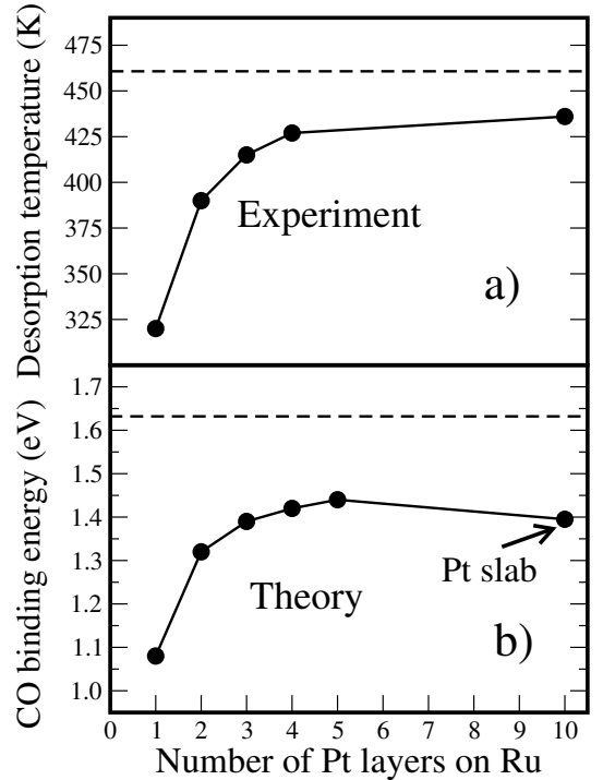
FIG. 3: CO interaction with Pt/Ru(0001) overlayer. a) experimentally determined desorption temperature; b) calculated CO binding energies. The dashed line denotes the corresponding result for pure Pt(111). The theoretical result for the largest number of Pt layers on Ru has been obtained by a calculation with a pure Pt slab with the lateral lattice constant of Ru (after [8]).
