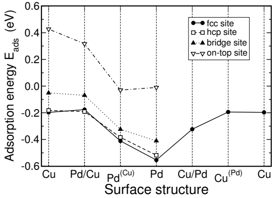
FIG. 5: Calculated atomic hydrogen adsorption energy on bimetallic PdCu surfaces for a quarter monolayer hydrogen coverage, namely on pure Cu(111), on a pseudomorphic Pd overlayer on Cu(111) (Pd/Cu), on pure Pd(111) with the lateral Cu lattice constant (Pd (Cu) ), on pure Pd(111), on a pseudomorphic Cu overlayer on Pd(111) (Cu/Pd), and on pure Cu(111) with the lateral Pd lattice constant (Cu (Pd) ) (after [10]).
