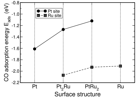
FIG. 6: Calculated CO adsorption energies at the top sites of Pt(111), Pt 2 Ru(111), PtRu 2 (0001) and Ru(0001) [6].
