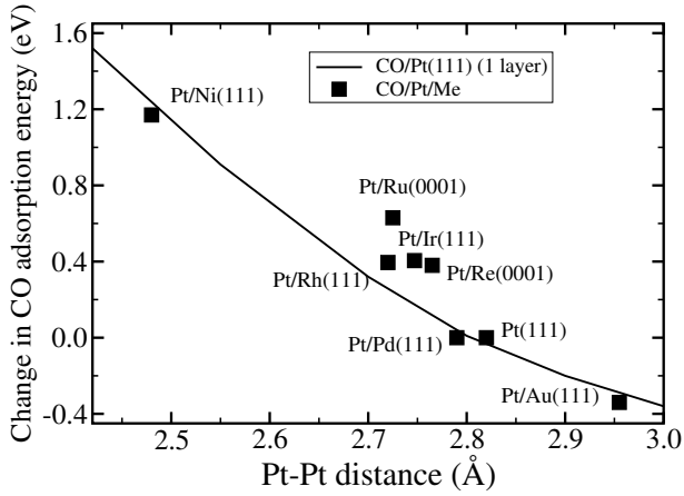
FIG. 2: Calculated change in CO adsorption energy with respect to CO/Pt(111) at the most stable adsorption site as a function of the Pt-Pt distance. A positive change in the adsorption energy means a reduced binding. The solid line corresponds to the CO adsorption energy in the hollow site of a Pt(111) one-layer slab (after [7]).
