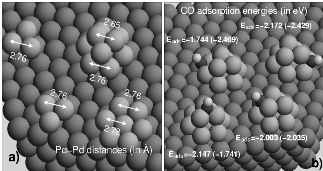
FIG. 9: Pd n cluster supported on Au(111) studied by DFT calculations. a) calculated nearest-neighbor Pd-Pd distances in Å of the Pd n cluster; b) CO adsorption positions and energies in eV on the Pd 10 /Au(111) cluster. The energies in parentheses correspond to the adsorption energies on free Pd 10 clusters in exactly the same configuration as the supported clusters (after [44]).
