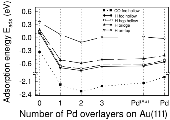
FIG. 4: CO and hydrogen adsorption energies as a function of the number of Pd overlayers on Au(111) for different adsorption sites on the surface at a coverage of \theta = 0.25 . The pure Pd substrates with the lateral lattice constant of Au ( a = 4.18 \text{ \AA} ) and Pd ( a = 3.96 \text{ \AA} ) are labeled by Pd (Au) and Pd, respectively (after [27]).
