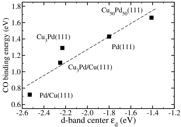
FIG. 7: Calculated CO binding energies on top of Pd atoms as a function of the local d -band center \epsilon_d . The dashed line is plotted as a guide to the eye (after [9]).
