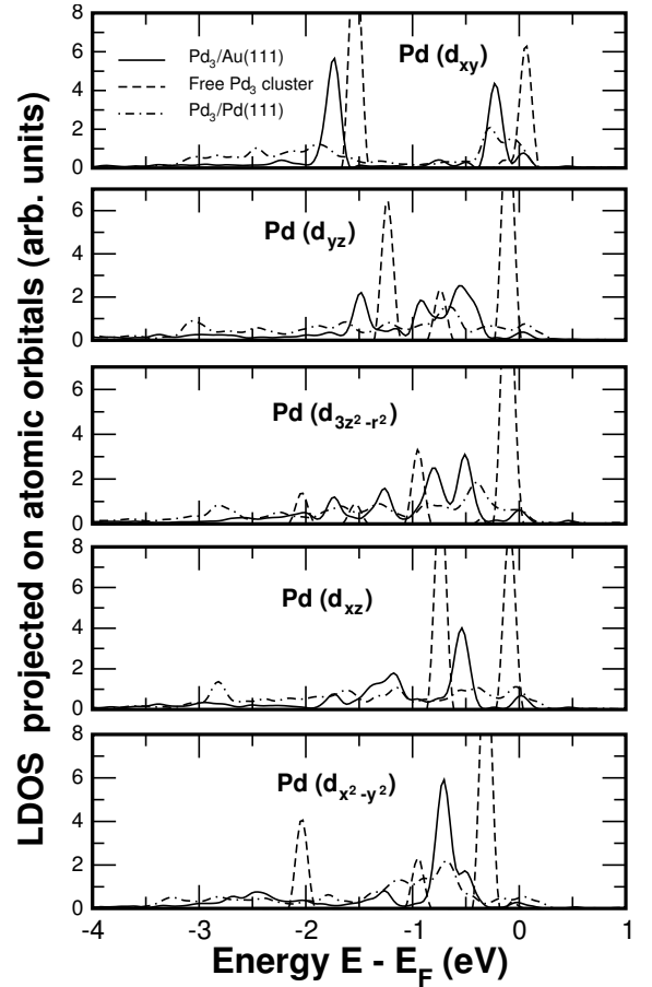
FIG. 10: Orbital resolved d -band local density of states (LDOS) of the supported Pd 3 /Au(111) and Pd 3 /Pd(111) clusters and the free Pd 3 clusters determined by DFT calculations (after [44]).
