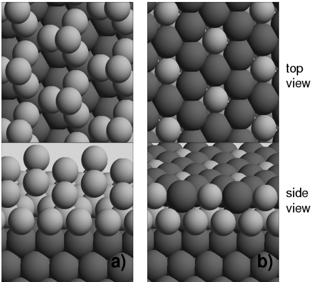
FIG. 11: Top and side view of two Mo/Au(111) structures studied by DFT calculations [65]. The dark and light balls represent Au and Mo, respectively.
