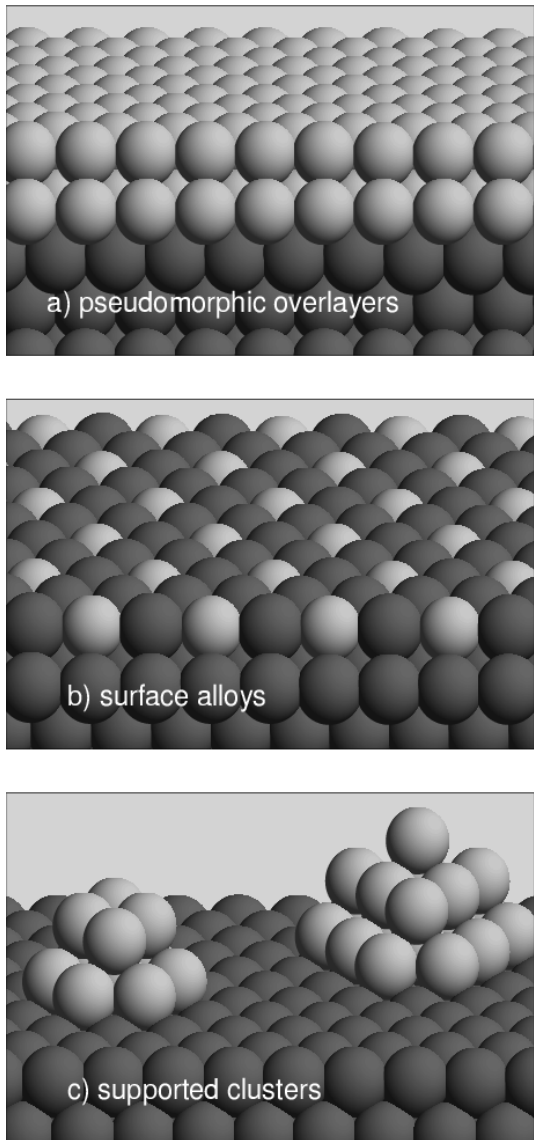
FIG. 1: Schematic illustration of the types of bimetallic systems discussed in this review.
