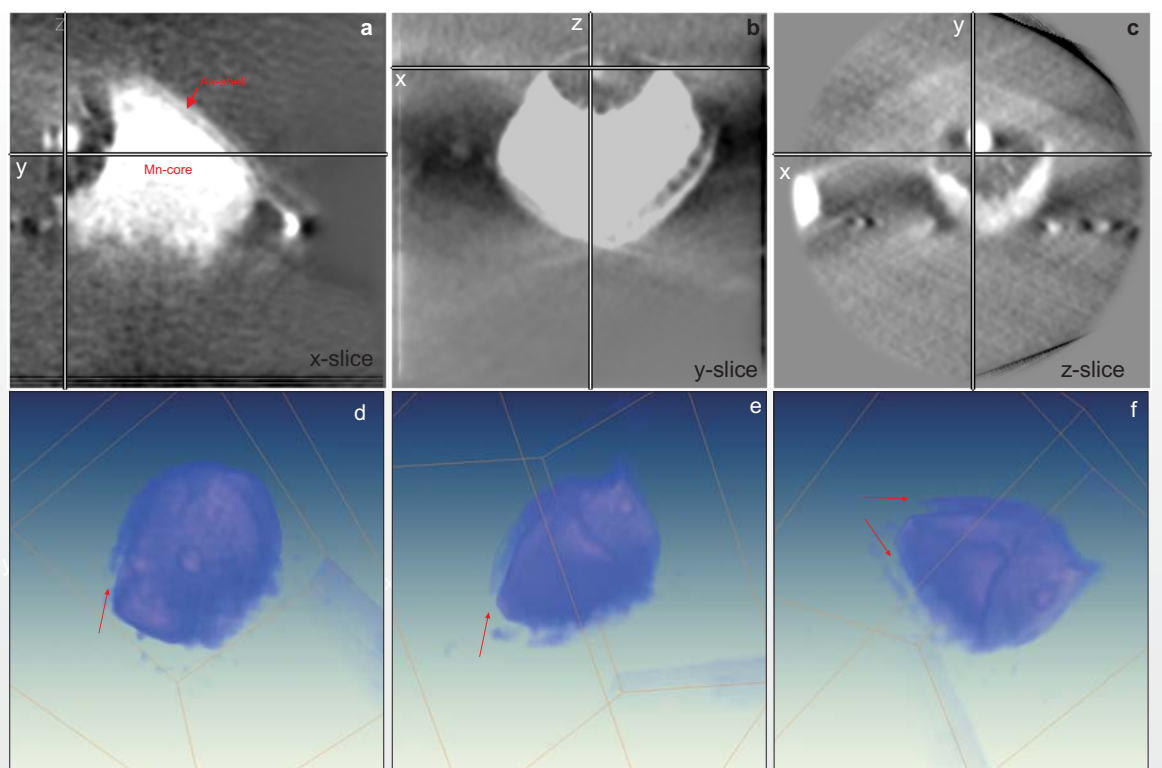
Figure 4. Reconstructed tomogram of the nanocrystal NC #1 shown in Fig. 3a. Fig. 4a,b,c are showing slice projections in x, y, z direction. Fig. d,e,f are volume renderings of the reconstructed structure. The nanocrystal has a core-shell structure (the arrows mark the boundary shell-core). Together with the EFTEM-results (Fig. 3b) it can be concluded that a crystalline Mn-rich core is surrounded by an amorphous As-rich shell. Mn [7] and As [8] have different diffusion constants in Si. The higher diffusion rate of Mn leads first to the formation of Mn-clusters in the voids and later then to an enrichment of As around the Mn-rich cluster. Further studies will investigate whether higher annealing temperatures and/or a different ion dose and ratio between Mn and As can change this fact.
