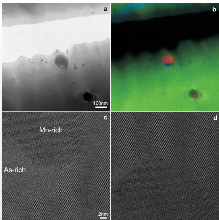
Figure 3. Fig. 3a shows a zero-loss (20eV) EFTEM image of the sample after annealing. Two Nanocrystals are specially marked. A composed map of EFTEM Mn (red), As (blue) and Si (green) images is shown in Fig.3b. NC #1 apparently consists of a separate Mn-rich and an As-rich phase. Fig. 3c shows a HRTEM image (taken at close to zero C_s ) of the interface Mn/As of NC #1. The Mn-rich phase of the nanocrystal is crystalline while the As-rich phase is amorphous. In Fig. 3d a HRTEM image of NC #2 is shown. Here the structure indicates a crystalline MnAs-nanocrystal without a separation of phases
