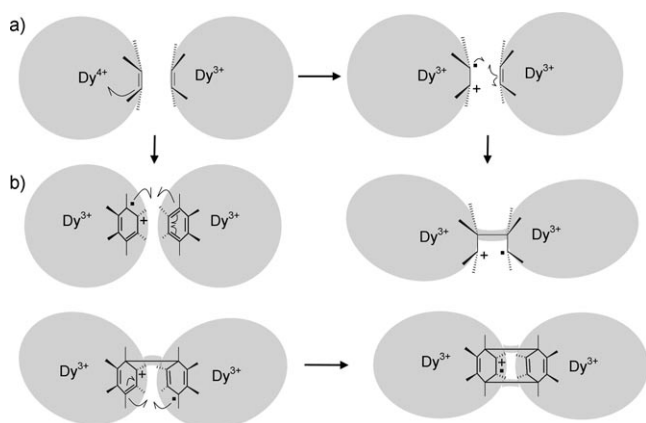
Figure 3. Proposed mechanisms for the initial stages of fullerene coalescence: a) \text{Dy}^{4+} withdraws an electron from one of the \text{C}=\text{C} bonds of fullerene, forming a radical cation that attacks another fullerene cage, which leads to the formation of \text{sp}^3 carbon atoms in the fullerene structures that cause the fullerene cages (gray) to distort. b) Alternatively, migration of the radical center may occur. The initial step is followed by a cascade of bond breaking and rearrangement of the fullerene cages driven by greater thermodynamic stability of the newly formed carbon nanotube.
