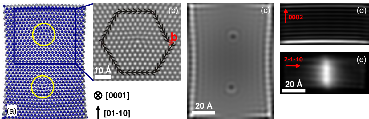
Figure 4. Atomic model for the edge a -type TD pair in Al(Ga) N (a) and calculated images (b-e) by applying the multislice algorithm on the model. In accordance with our TEM measurements, the HRTEM calculation identifies the dislocation as a pure edge a -type TD with \mathbf{b} = 1/3 [2-1-10] (b). In the [0001] BF calculation the dislocation pair is clearly visible, as it was observed in our plane-view TEM investigations (c). Also the WBDF calculations and the verification of the \mathbf{g} \cdot \mathbf{b} criterion are consistent with the experiment (d, e).
