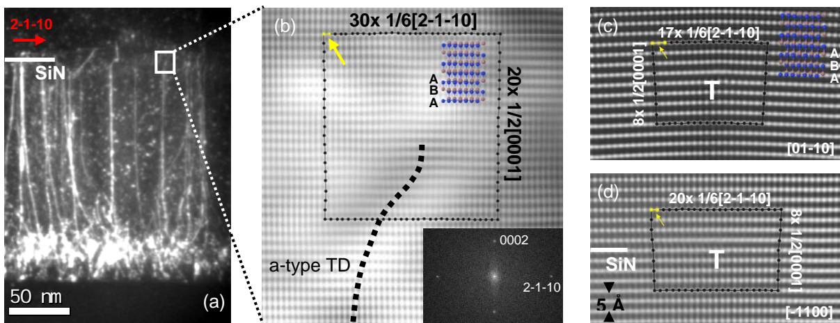
Figure 6. Burgers vector analysis of an annihilated pure edge a -type TD (a) at the SiN x interlayer and comparison with HRTEM multislice calculations. The unclosed Burgers TD circulation in the filtered HRTEM image (b) results in a Burgers vector of 1/6[2-1-10] in the imaged projection. Thus, the dislocation line of the TD gets a component perpendicular to the image plane at the SiN x interface. The unclosed circulation in the calculated image at the [01-10] zone (c) shows the Burgers vector 1/3[2-1-10] of the a -type basal dislocation, as provided in the model. In accordance to (b) we receive a Burgers vector of 1/6[2-1-10] in the calculated image from the [-1100] zone, corresponding to the imaging of the a -type Burgers vector from a 60° projection.
