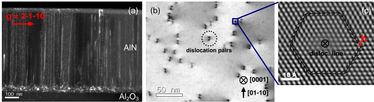
Figure 3. Cross-sectional WBDF image of S2 shows pure edge a -type TDs in AlN (a). In the [0001] plane-view image the arrangement of the a -type TDs in pairs along the [01-10] direction is clearly visible (b). This dislocation structure exactly corresponds to the Volterra cut along the [01-10] direction. The unclosed Burgers circulation around the dislocation core in the Fourier filtered HRTEM micrograph definitely identifies the TD as a pure edge a -type TD with Burgers vector \mathbf{b} = 1/3 [2-1-10] (c).
