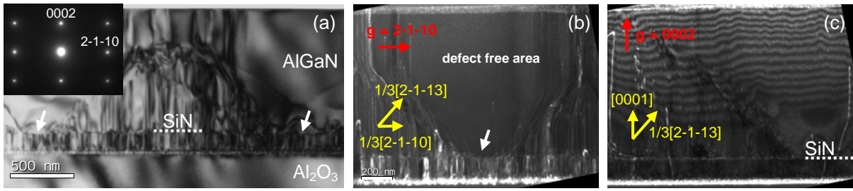
Figure 1. TEM cross-sectional views of sample S1. The BF image (a) from the [01-10] zone axis shows regions of the \text{SiN}_x layer at which the dislocation annihilation is highly efficient (bottom arrows in (a) and (b)), whereas the propagation of the TDs is not stopped in other regions. The WBDF images are recorded from the same sample area, exploiting the 2-1-10 (b) and the 0002 reflection (c). The Burgers vectors of the TDs visible in the respective WBDF image are also charted. In general, the sample shows a very high density of pure edge a -type TDs beneath the \text{SiN}_x layer (b), whereas the number of screw and mixed TDs is very small (c). Thus the appearance of large defect free areas is primarily based on the bending and annihilation of the pure edge a -type TDs at the \text{SiN}_x layer.
