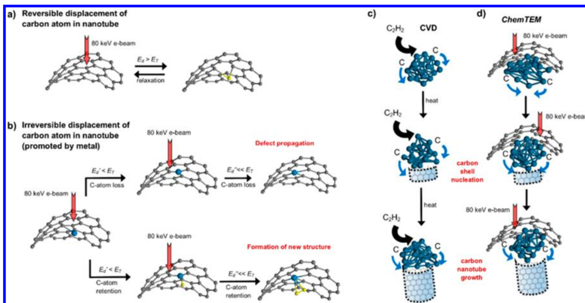
Figure 1. (a) 80 keV electron beam of TEM supplies kinetic energy to carbon atom ( E_T ) insufficient to overcome the barrier for irreversible displacement ( E_d ). However, (b) in the presence of metal atom inside the nanotube, the barrier is lower ( E_d' ) such that C atoms are selectively removed from SWNT in vicinity of the metal, either leaving the system (top) or remaining adsorbed on the metal (bottom, adsorbed C atoms are highlighted yellow). The carbon atoms displacement from SWNT and retention on metal leads to formation of new structures inside nanotube. A comparison of nanotube formation in CVD (c) with ChemTEM (d) demonstrates that reactive carbon atoms are formed via metal-catalyzed decomposition of molecules or carbon nanotube sidewall respectively, in both cases leading to diffusion of carbon atoms across the nanocatalyst to form a new nanotube structure (outlined with dotted lines).
