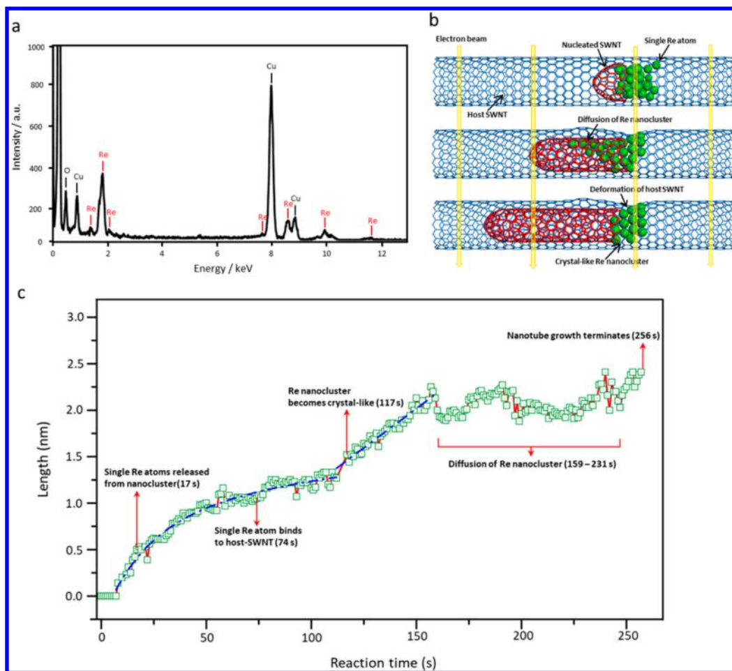
Figure 3. (a) EDX spectroscopy confirms the identity of the metal clusters within the SWNT as Re (Cu peaks are due to the TEM specimen grid). (b) Schematics of the e-beam stimulated SWNT growth catalyzed by Re nanocluster. (c) Plot showing the changing length of the growing nanotube measured by AC-HRTEM as a function of time. The growth starts from 7 s. The exponential decay function from 7 to 112 s includes the nucleation stage (7–17 s) and growth stage 1 (17–112 s). The linear increase from 113 to 159 s is growth stage 2. Blue dashed lines are fitted by an exponential decay function and a linear equation, respectively. The key events during the growth of the SWNT are highlighted by red arrows. The error in the measured length for each data point is \pm 0.03 nm due to the size of the pixels in the individual TEM images; the error of the reaction times given for each data point is \pm 1.0 s due to the exposure time used.
