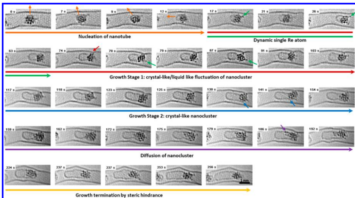
Figure 2. Time series of AC-HRTEM images following the formation of a carbon nanotube on a nanocluster of Re embedded within a host-SWNT (Re@SWNT). Orange, green, red, blue, and purple short arrows indicate the direction of nanotube nucleus formation (carbon shell), positions of dynamic single Re atoms, single atom contact sites in nanotube, newly nucleated SWNT wall, and diffused Re atoms, respectively.
