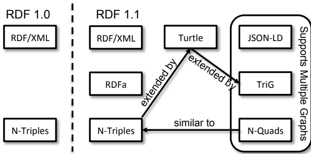
Fig. 5 RDF serialization formats
