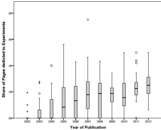
Fig. 12 Box-plot showing the relative number of pages of Category 2 (Design and Modeling) papers by year of publication. The median starting at 0% in 2002 increases constantly (with the exception of 2010) over time, reaching its top of 24% in 2012. The second/third quartile, denoted by the box, varies, but is since 2009 clearly above zero. Outliers are displayed as circles/stars. (taken from [44])
