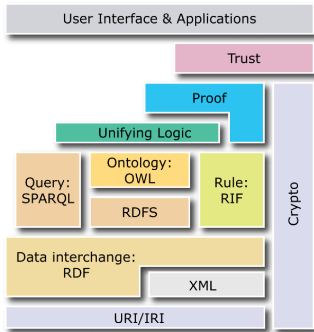
Fig. 3 The Semantic Web architecture Copyright ©World Wide Web Consortium, (MIT, ERCIM, Keio, Beihang) http://www.w3.org/Consortium/Legal/2015/doc-license
