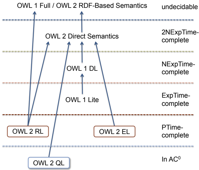
Fig. 9 Worst-case complexities of the different OWL sub-languages
