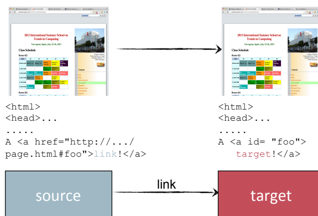
Fig. 1 Plain links between HTML pages
