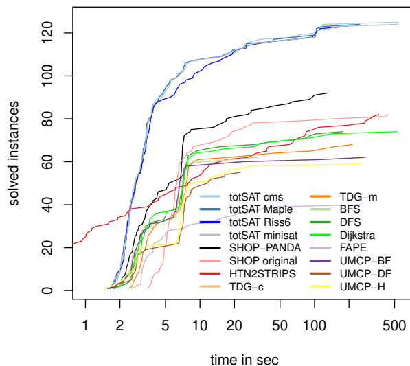
Figure 2: Runtime vs number of solved instances per planner
