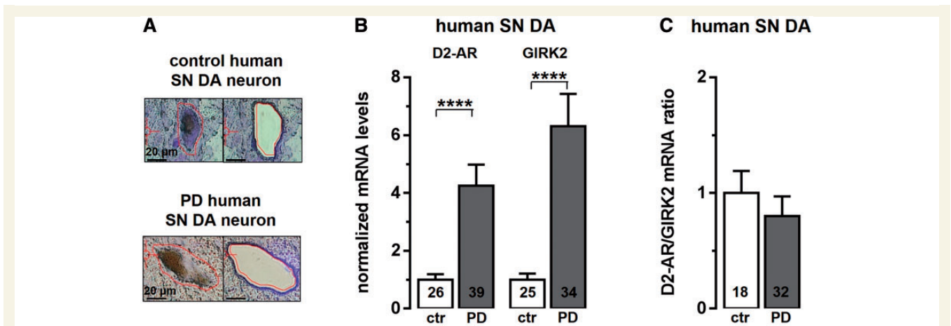
Figure 1 Elevated D2-autoreceptor (AR) and GIRK2 messenger RNA levels in remaining human SN DA neurons from patients with Parkinson's disease (PD). (A) Neuromelanin-positive human SN DA neurons (SN DA) (before and after UV laser microdissection) from post mortem Parkinson's disease and control midbrain sections (for details, see Supplementary Table 1 ). (B) Real-time quantitative PCR results identified significantly higher relative messenger RNA levels for D2-autoreceptors and GIRK2 in human SN DA neurons from Parkinson's disease brains compared to controls (ctr) (D2-autoreceptors: controls, n = 26 , 1 \pm 0.19 ; Parkinson's disease, n = 39 , 4.25 \pm 0.73 ; ****P < 0.0001 ; Mann-Whitney test; GIRK2 : controls, n = 25 , 1 \pm 0.25 ; Parkinson's disease, n = 34 , 6.31 \pm 1.12 ; ****P < 0.0001 ; Mann-Whitney test). (C) D2/GIRK2 ratios were not different in SN DA neurons from controls and Parkinson's disease patients. All data are shown as the mean \pm SEM.
