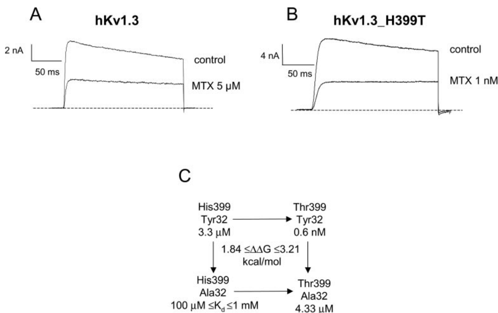
Fig. 8. Comparative block of MTX on currents through wild-type (A) and mutant (B) hKv1.3 channels. The original current traces through hKv1.3 channels represented in the figures were measured in transiently transfected COS-7 cells and elicited by 200-ms depolarizing voltage steps, from the membrane potential -80 to +40 mV, every 40 s. C, thermodynamic mutant cycle performed for MTX_Tyr 32 and hKv1.3 His 399 . The K_d values were calculated using dose-response or single concentrations (when K_d values were greater than 100 nM) as described under Materials and Methods . The changes in coupling energy ( \Delta\Delta G ) for wild-type and mutant MTX and hKv1.3 channels were calculated using the K_d values of the wild-type and mutant MTX and hKv1.3 channels (see Materials and Methods ).
