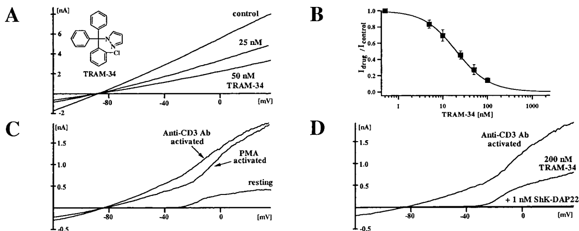
Fig. 3. (A) IKCa1 currents in COS-7 cells blocked by TRAM-34. (B) Dose response for IKCa1 channel block by TRAM-34. The Hill equation was fitted to the reduction of slope conductance at -80 mV (15 cells). (C) IKCa currents in resting human T lymphocytes and in T lymphocytes activated for 2 days with PMA or anti-CD3 Ab. Mean IKCa conductance in resting cells = 0.098 (±0.17) ns ( n = 24), PMA activated (10 nM) = 3.45 (±2.21) ns ( n = 21), anti-CD3 Ab-activated (5 ng/ml) = 5.59 (±3.91) ns ( n = 20). (D) Effect of TRAM-34 and ShK-Dap 22 on K + currents in activated T lymphocytes.
