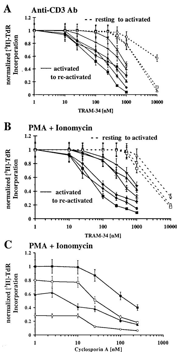
Fig. 4. Effect of TRAM-34 on anti-CD3 Ab- (A) or PMA + ionomycin- (B) stimulated [ ^3 H]-TdR incorporation by resting and preactivated lymphocytes. PBMCs from different donors were activated with anti-CD3 Ab (5 ng/ml) or a combination of PMA (10 nM) + ionomycin (175 nM) for 48 h. [ ^3 H]TdR was added to the culture for the last 6 h. In parallel, PBMCs were preactivated with either anti-CD3 Ab (5 ng/ml) or 10 nM PMA for 48 h (to up-regulate IKCa1 channels) and then restimulated for a further 48 h with anti-CD3 Ab or PMA + ionomycin. Donor 1 resting (□), donor 2 resting (○), donor 3 resting (Δ), donor 1 preactivated (■), donor 2 preactivated (●), donor 3 preactivated (▲), donor 4 preactivated (◆), donor 5 preactivated (X), donor 6 preactivated (–). (C) Effects of TRAM-34 on cyclosporin A-mediated inhibition of [ ^3 H]-TdR incorporation. PBMCs from donor 1 were preactivated with 10 nM PMA for 48 h and then restimulated for a further 48 h with PMA + ionomycin in the presence or absence of cyclosporin A and TRAM-34. [ ^3 H]TdR was added to the culture for the last 6 h. Cyclosporin (CsA) alone (■), CsA + 250 nM TRAM-34 (□), CsA + 500 nM TRAM-34 (▲), CsA + 1 \mu M TRAM-34 (○).
