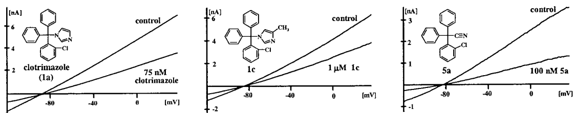
Fig. 1. Inhibitory effects of compounds 1a (clotrimazole), 1c , and 5a on IKCa1 currents expressed in COS-7 cells. Voltage ramps were applied from -120 mV to 40 mV.
