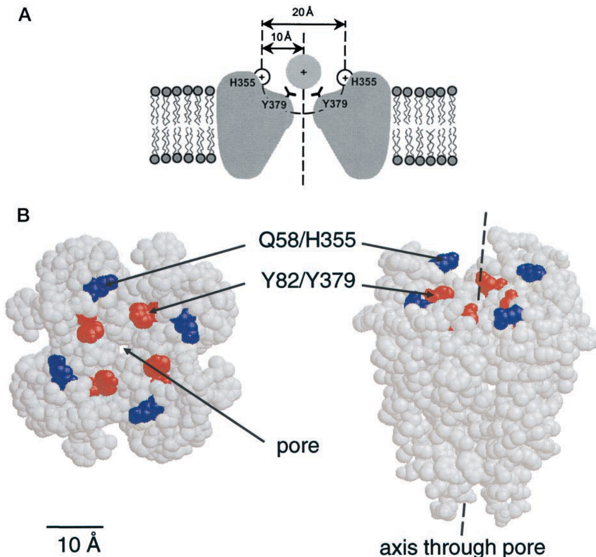
FIGURE 7 Proposed interaction of amino acid residues and \text{TEA}^+ . (A) Diagram of the external vestibule of a Kv1.1 channel illustrating the interactions between [\text{TEA}^+]_o and H355. (B) Surface view of the KcsA channel from the top (left) and slightly tilted (right) using RasMol (version 2.6). Q58 of the KcsA channel, equivalent to H355 in Kv1.1 (F425 in Shaker ), is shown in blue. Y82 of the KcsA channel, the equivalent of Y379 in Kv1.1 (T449 in Shaker ) is shown in red.
