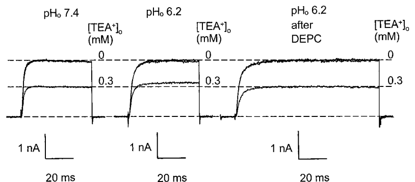
FIGURE 4 Influence of DEPC treatment on [\text{TEA}^+]_o block of current through \text{Kv}1.1 channels. Whole-cell currents of one cell were elicited by 50- or 100-ms depolarizing voltage steps to 40 mV and are shown before, during, and after the application of 0.3 mM \text{TEA}^+ at \text{pH}_o 7.4 (left), at \text{pH}_o 6.2 (middle), and at \text{pH}_o 6.2 after washout of 500 \mu\text{M} DEPC (cell was treated with DEPC for 5 min at \text{pH}_o 6.2; right).
