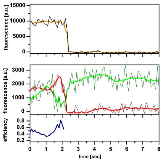
Fig. 3. Alternating laser excitation. The graph shows an exemplary time trace of the DNA1–RNA26 sample. The excitation laser was alternated frame by frame between 633 nm (direct–acceptor excitation, Upper ) and 532 nm (FRET excitation, Lower ) (34). Actual data and a 10-point sliding average are shown as thin and thick lines, respectively.
