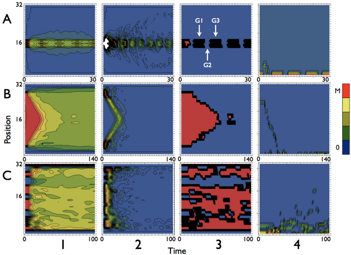
Fig. 2: (Colour on-line) From left to right: Countour plot of the time evolution of the populations \langle n_i(t) \rangle (column 1), visibility v_i(t) (column 2), discretized populations \mathcal{D}_i(t) (column 3) and clustering \mathcal{C}(\ell, t) (column 4) for three different initial configurations: four alive sites separated by two dead ones (A), twenty-four alive sites grouped together (B) and a random initial configuration (C). Time is reported on the x -axis (in arbitrary units), and position (cluster size) i = 1, \dots, L on the y -axis in columns one to three (four). Arrows in panel 3A highlight the three subsequent generations of a “blinker” reported schematically in fig. 3. The colour code goes from zero to M = 1 ( M = 4 for the clustering and to M = .1 for the visibility), from blue through green to red.
