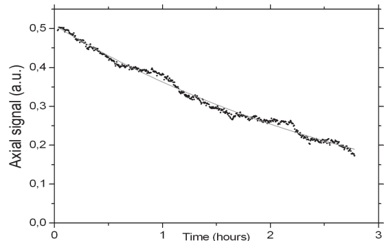
Fig. 3. Evolution of the axial signal during a resonant drive. The signal decays exponentially with a time constant of 3.5 hours.
