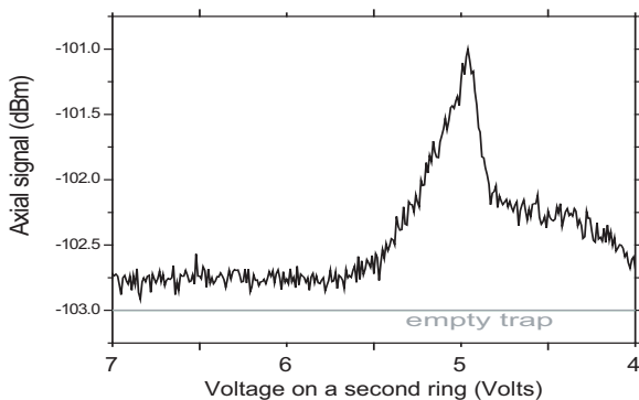
Fig. 4. Observation of an axial signal during a scan of the voltage on the second ring ( U_2 ). Electron energy distributed over a large energy band. The solid gray line corresponds to the signal when no electrons are present in the trap.
