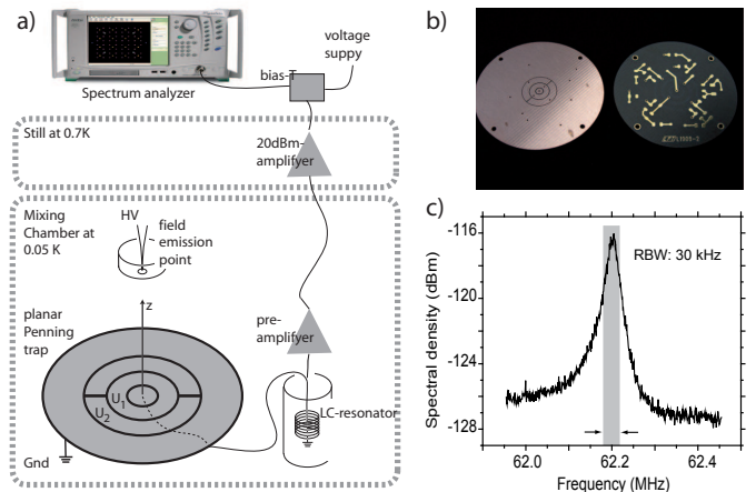
Fig. 1. a) Sketch of the experimental setup: The planar trap consists of a central circular electrode on ground potential surrounded by two rings at voltages U_1 and U_2 . The signal from the central electrode is resonantly enhanced, amplified in two stages and recorded on a spectrum analyzer. b) Photo of the front and back side of the planar Penning trap used in the experiment. c) Noise spectrum of the LC-circuit taken at T \simeq 100 mK. A resolution bandwidth of 30 kHz is indicated by a grey bar, this setting was used for the experiments described below.
