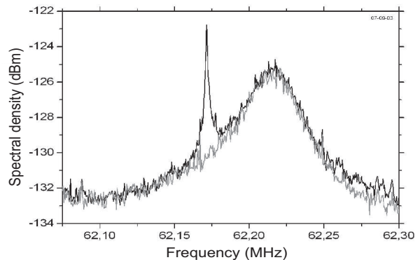
Fig. 5. Spectral noise of a tuned LC-circuit. The black line shows the response of electrons cloud to the parametric drive applied to one of the electrodes of the planar trap. For comparison a scan without trapped electrons, showing the empty resonance of the tank-circuit (grey line).
