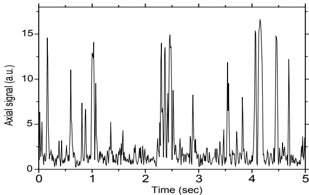
Fig. 6. Time evolution of the amplitude of the parametric resonance. Clearly separated bursts are likely being associated with the excitation of only a few electrons. RBW = 30 Hz.
