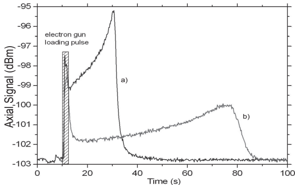
Fig. 2. Loading and trapping of clouds of electrons at different values of potential U_1 . The data (a) were recorded at U_1=5.2\text{V} , (b) at U_1=4.8\text{V} . The RBW was set to 30 kHz.
