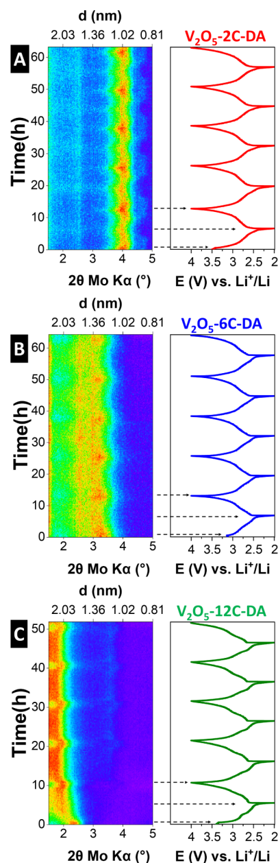
Figure 7. Electrochemical (de)lithiation mechanism studied via operando XRD (Mo K\alpha X-ray source, \lambda = 0.71 \text{ \AA} ) using a Debye–Scherrer (transmission) geometry in modified coin cells versus lithium metal over five consecutive galvanostatic charge/discharge cycles at a specific current of 50 mA/g. (A) \text{V}_2\text{O}_5 -2C-DA, (B) \text{V}_2\text{O}_5 -6C-DA, and (C) \text{V}_2\text{O}_5 -12C-DA.
