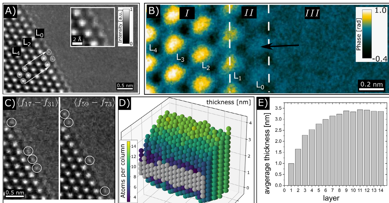
FIGURE 2 | Analysis of surface dynamics and specimen thickness. (A) Time average of in situ HR-TEM series from the Pt (111) surface in H 2 O. Dynamic surface regions L 0 show a blurred contrast. (B) Averaged reconstructed phase signal. The image in (B) is color-coded to represent the platinum columns in yellow. For this lateral averaging the super cell was defined as an area of 2 nm × 0.7 nm, which contains periodically repeated information of seven super cells. Region I shows the atomic columns of bulk platinum. The thickness decreases toward the surface, layers are counted from the surface. The phase signal at L 0 corresponds to the dynamic layer in (A), showing a higher signal at FCC positions as highlighted by the circles in (A) and the black arrow. (C) Subset time average of 14 frames (5.6 s) of the in situ movie at different initial times (frame sets). The most intense columns in the dynamic surface layer L 0 are marked to guide the eye. The position-change of these signals indicates mobile platinum ad-atoms. (D) The number of atoms in a specific column is determined by averaging the phase signal in a unit cell around the column and compared to simulations, resulting in the surface model. Surface atoms in L 1 are marked in gray color. (E) The average layer thickness profile starting from L 1 .
