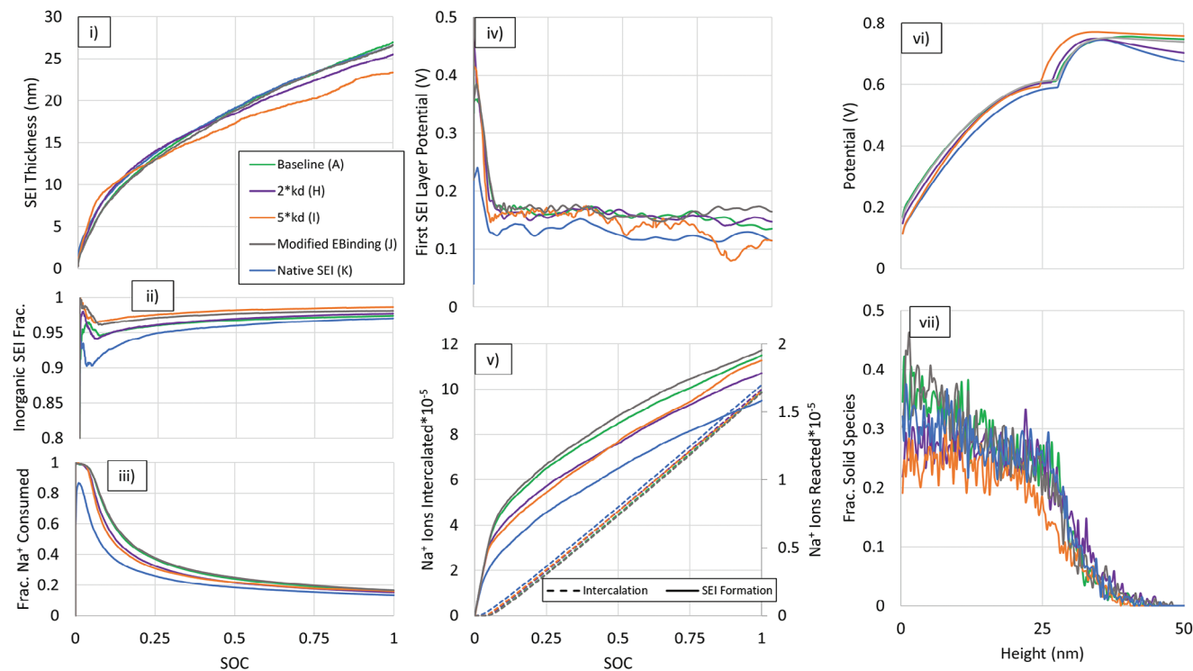
Figure 4. Impact of diffusion and native SEI (systems A/H/I/J/K) on SEI growth and properties during a full charge. i) SEI thickness, ii) mole fraction of the SEI that is inorganic, iii) molar fraction of \text{Na}^+ consumed for SEI formation, iv) the potential of first SEI layer at the electrode surface, v) amount of \text{Na}^+ ions consumed by intercalation and SEI formation reactions, vi) spatial potential of each system at SOC = 1, and vii) fraction of solids at a given height at SOC = 1.
