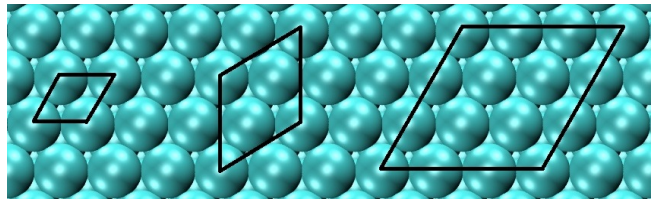
FIG. 1. Illustration of the unit cells used to represent the surface structures. Left: (1 \times 1) , Center: R30^\circ(\sqrt{3} \times \sqrt{3}) . Right: (3 \times 3) , mainly used to model the different Pd ensembles in PdAg/Pd(111) surface alloys.
