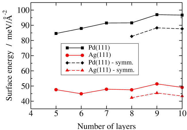
FIG. 2. Surface energies in \text{meV}/\text{\AA}^2 for Pd(111) and Ag(111). Asymmetric and symmetric slabs with different number of layers at the PBE/PAW level of theory. For asymmetric slabs three layers are relaxed at one side. For symmetric slabs three layers are relaxed at each side.
