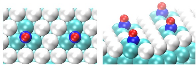
FIG. 8. Adsorption of CO on a hollow site of Pd 3 ensembles at the PdAg/Pd(111) surface alloy. Left: The pure monolayer alloy. Right: The topmost monolayer alloy with underlying silver layers.
