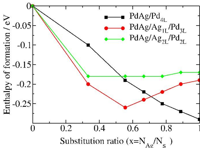
FIG. 4. Surface alloy enthalpies of formation \Delta H , in eV, for the \text{Pd}_{(1-x)}\text{Ag}_x/\text{Ag}_{nL}/\text{Pd}(111) structures as a function of the substitution ratio x . The index nL denotes a certain number of silver layers between Pd(111) and the surface alloy. The substitution ratio x accounts for the number of palladium atoms replaced by silver atoms at the topmost layer.
