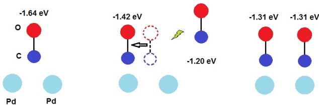
FIG. 9. Simplified illustration of CO adsorption on a Pd 2 ensemble under high CO exposure conditions. Left: Preferred adsorption at the bridge site. Center: Energetics relevant for the additional adsorption of a CO molecule on a Pd 2 dimer. Right: Simultaneous adsorption at the top sites.
