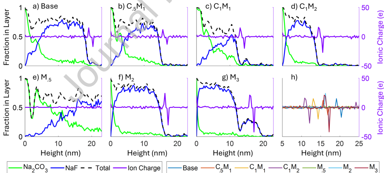
Figure 5: Visualization of EDL and SEI composition over HC surface at 100% SOC after first charge for selected systems. a-g) Fractional SEI composition and ionic charge (number of \text{Na}^+ - number of \text{PF}_6^- ) of vs height. h) The ionic charges of all systems overlayed together. C subscripts correspond to C-rate, and M subscripts correspond to molar \text{NaPF}_6 concentration in the electrolyte. Further system details are available in Table 1.
