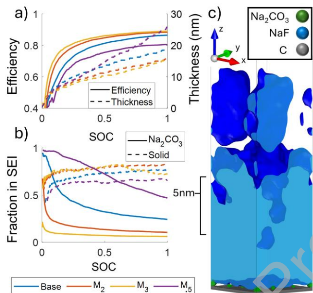
Figure 3: SEI evolution and properties during first charge at 0.25C in systems in systems with varied \text{NaPF}_6 concentration. a) Coulombic efficiency and SEI thickness, b) Fraction of \text{Na}_2\text{CO}_3 and solid species in SEI, for systems with varied salt concentration. c) The SEI formed at 100% SOC in the 3 molar \text{NaPF}_6 system. Subscripts correspond to molar concentration of \text{NaPF}_6 in the electrolyte. Additional system information is available in Table 1. Solvent, salt, and intermediate species are removed for ease of visualization.
