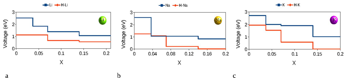
Fig. 8 Discharge curves for the insertion of (a) Li, (b) Na, and (c) K in the lignin-derived (C-lignin- \alpha ) polymer model structure. Voltage curves are only shown for the structure that was created at 1273 K (see Fig. 1c). X denotes the concentration of inserted atoms in the investigated model systems (X corresponds to the number of inserted AM atoms divided by the total number of atoms). H-AM shows the AM concentration in a hydrogen-saturated mode system, HC-lignin- \alpha .
