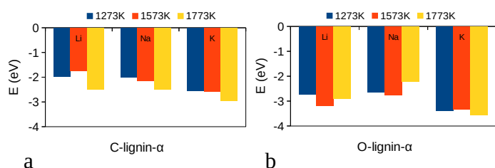
Fig. 4 : The most favorable sites for insertion of a single AM atom regarding the C-lignin- \alpha and O-lignin- \alpha .
