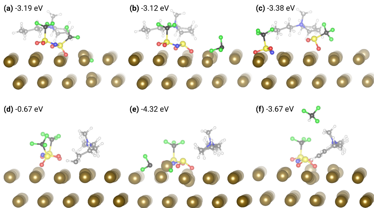
Figure 5. Structures of possible initial decomposition products of BMP-TFSI on Na(0001), obtained upon breaking a C-F bond (a), an S-C bond (b) and an N-S bond (c) of TFSI, or an N-C bond of BMP (d). In the decomposition product shown in panel (e), both an S-C and a C-F bond of TFSI are broken. Finally, in the structure shown in panel (f) both BMP and TFSI are decomposed and gaseous \text{CH}_3\text{F} is formed. The respective reaction energies are given with respect to that of the intact BMP-TFSI ion pair adsorbed on Na(0001).
