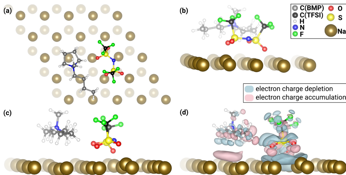
Figure 4. Top view (a) and side views (b-d) of the adsorption structure of BMP-TFSI within a (5x5) overlayer structure on Na(0001). In (d) the charge rearrangement due to adsorption of BMP-TFSI on Na(0001) is shown. Two isosurfaces (values of \pm 0.001 \text{ e}/\text{\AA}^3 ) of the electron density difference between the electron densities of the adsorption complex and the isolated BMP-TFSI and the bare Na(0001) surface are depicted.
