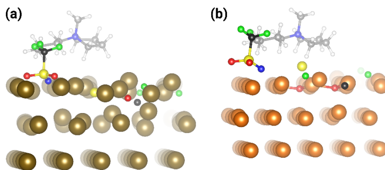
Figure 6. Structures due to further decomposition steps to, in parts, atomic adsorbates on the Na(0001) surface (a, reaction energy: -11.79 eV) and for comparison on the Mg(0001) surface (b, reaction energy: -12.35 eV). [26]
