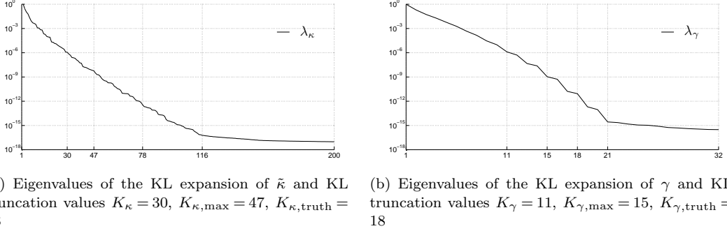
FIGURE 6.5. Eigenvalues and truncation values of the Karhunen-Loève expansions
