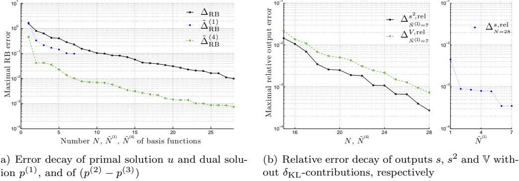
FIGURE 6.6. Greedy error decay
