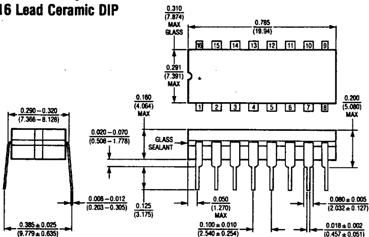
N Package 16 Lead Plastic DIP
